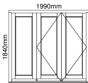
Door Standard Door 50mm thick Timber Type: Accoya
