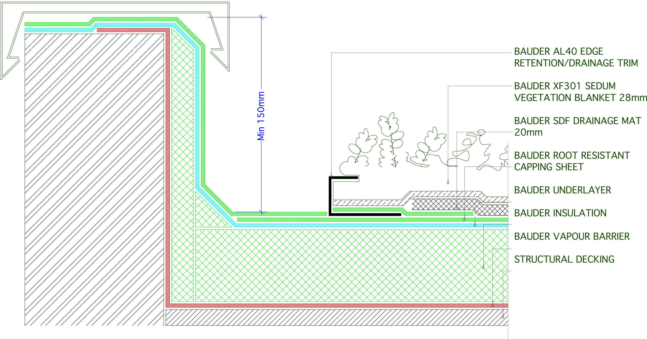
UPSTAND DETAIL TO INSULATED PARAPET WALL WITH METAL CAPPING / AL40 EDGE RETENTION/DRAINAGE TRIM OPTION
