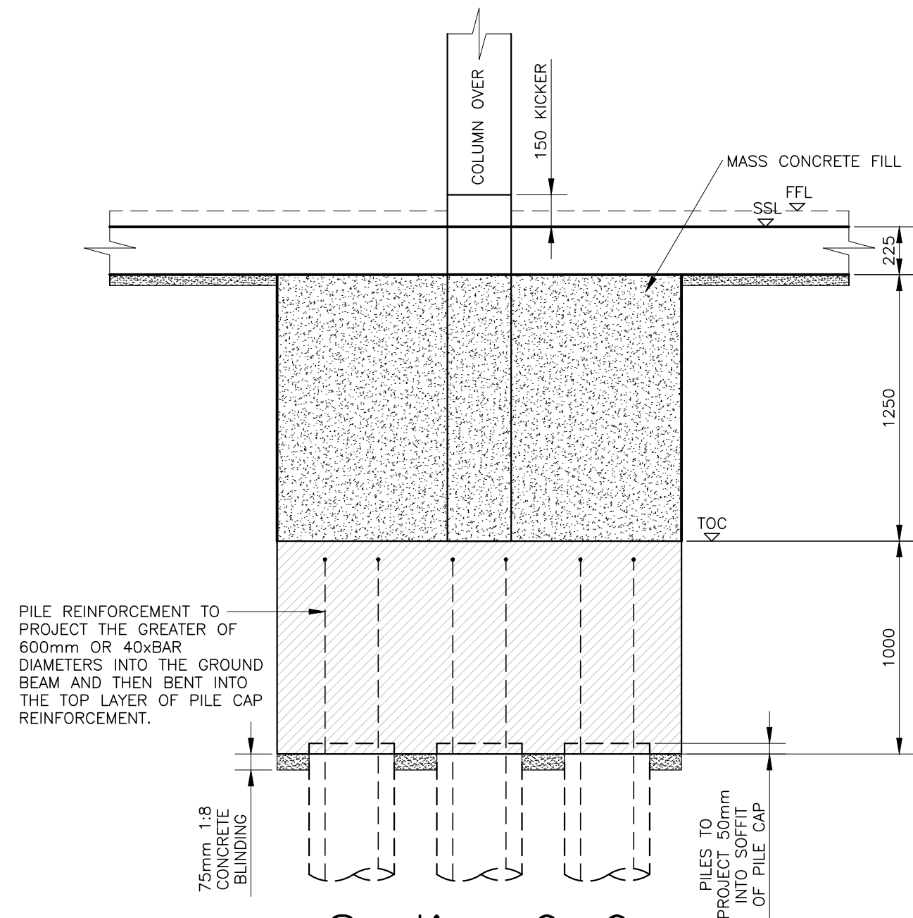
Section 9-9 Scale 1:25
