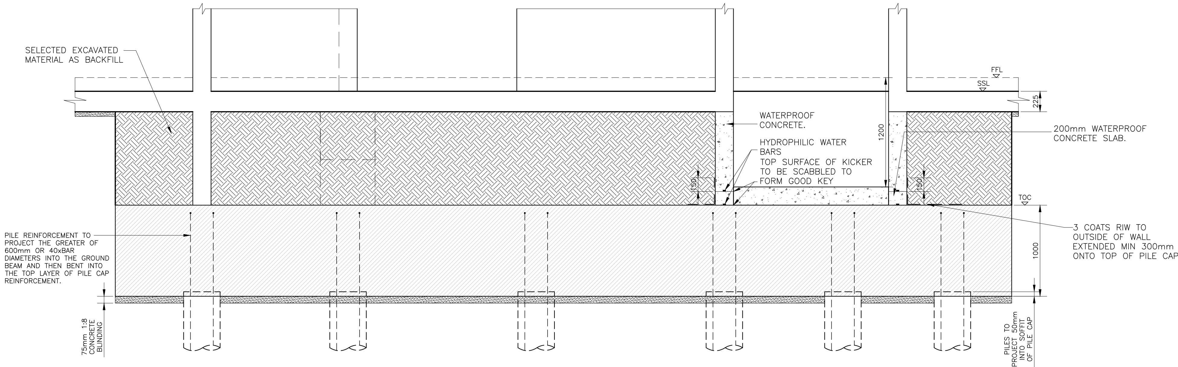
Section 10-10 Scale 1:25
