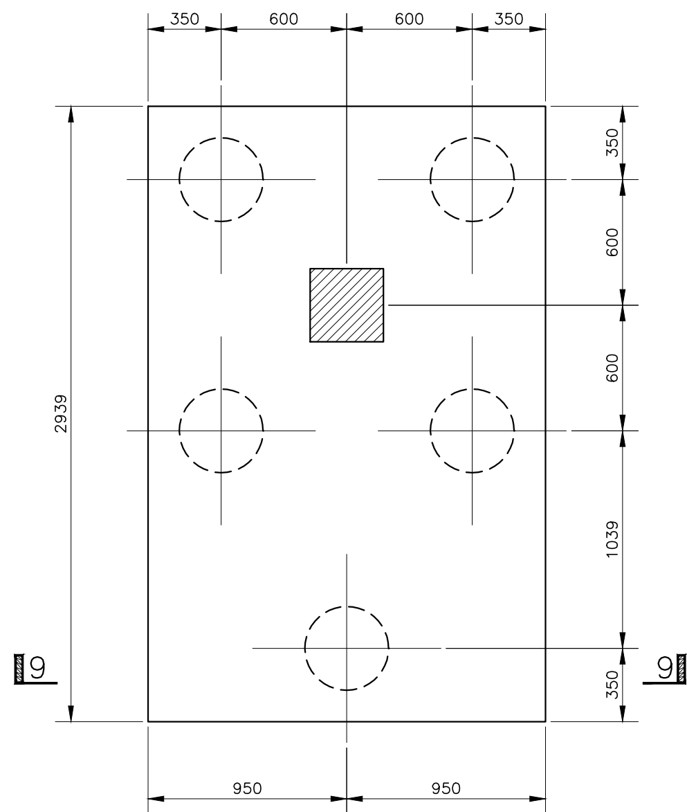
P05 Pile Cap Scale 1:25
