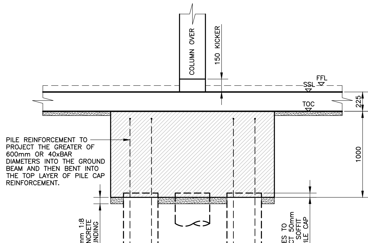
Section 3-3 Scale 1:25
