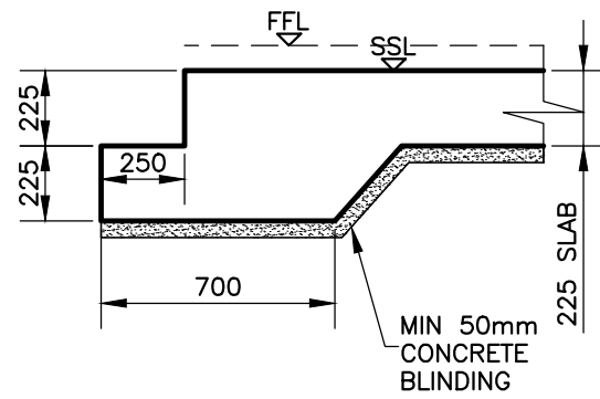
Typical Slab Edge Detail Scale 1:25
