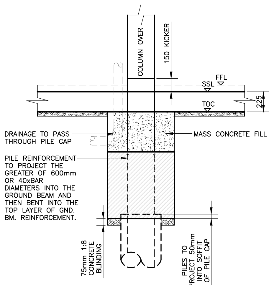
Typical Section at SVP Scale 1:25
