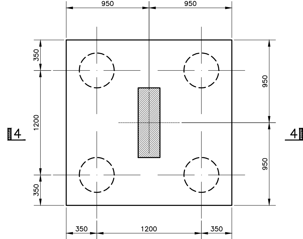
P04 Pile Cap Scale 1:25
