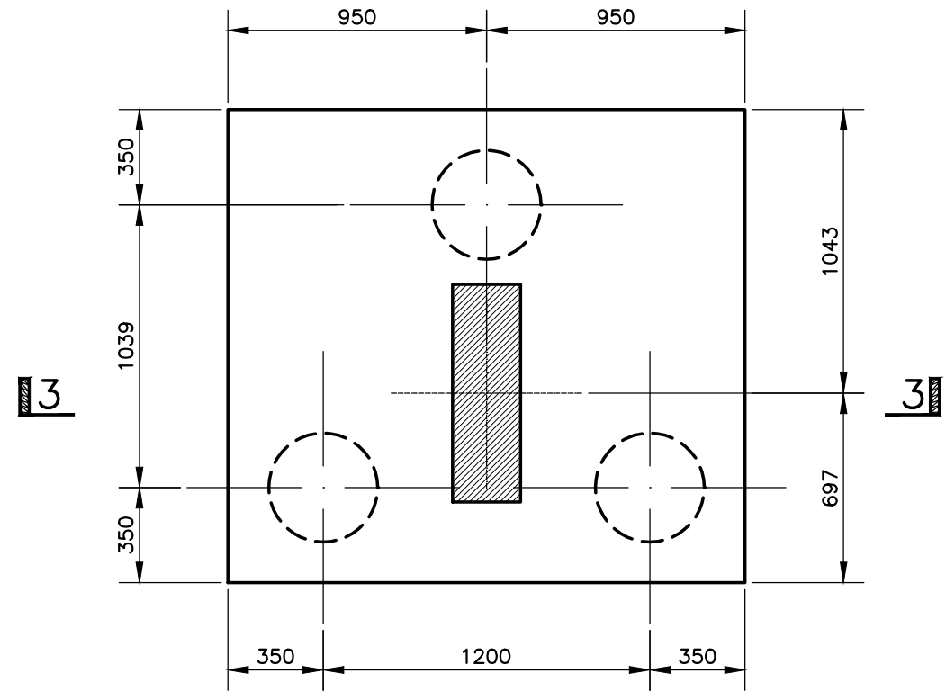
P03 Pile Cap Scale 1:25
