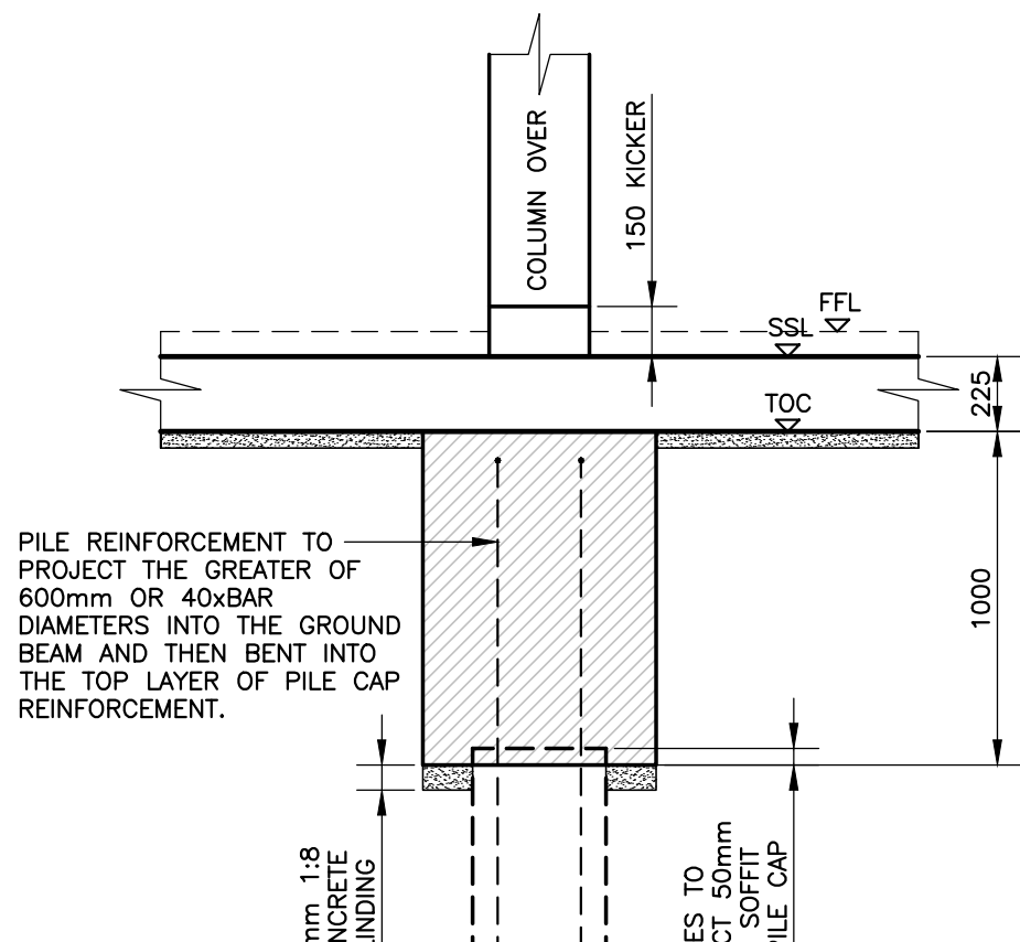
Section 2-2 Scale 1:25
