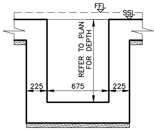
Typical Manhole Section Scale 1:25
