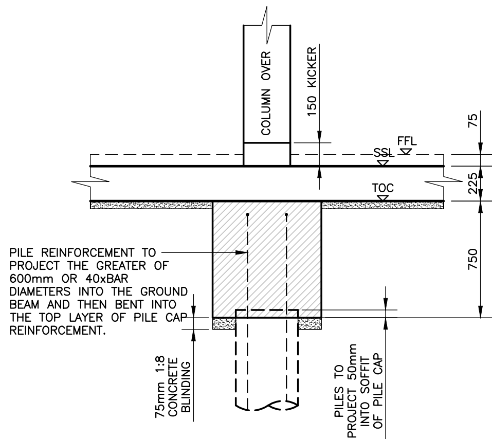
Section 1-1 Scale 1:25
