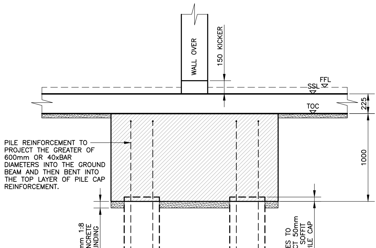
Section 4-4 Scale 1:25
