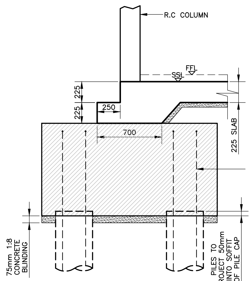
Typical Slab Edge Detail at Pile Cap Scale 1:25
