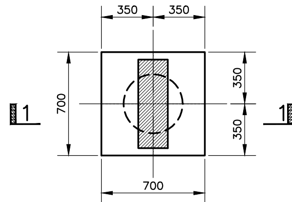
P01 Pile Cap Scale 1:25
