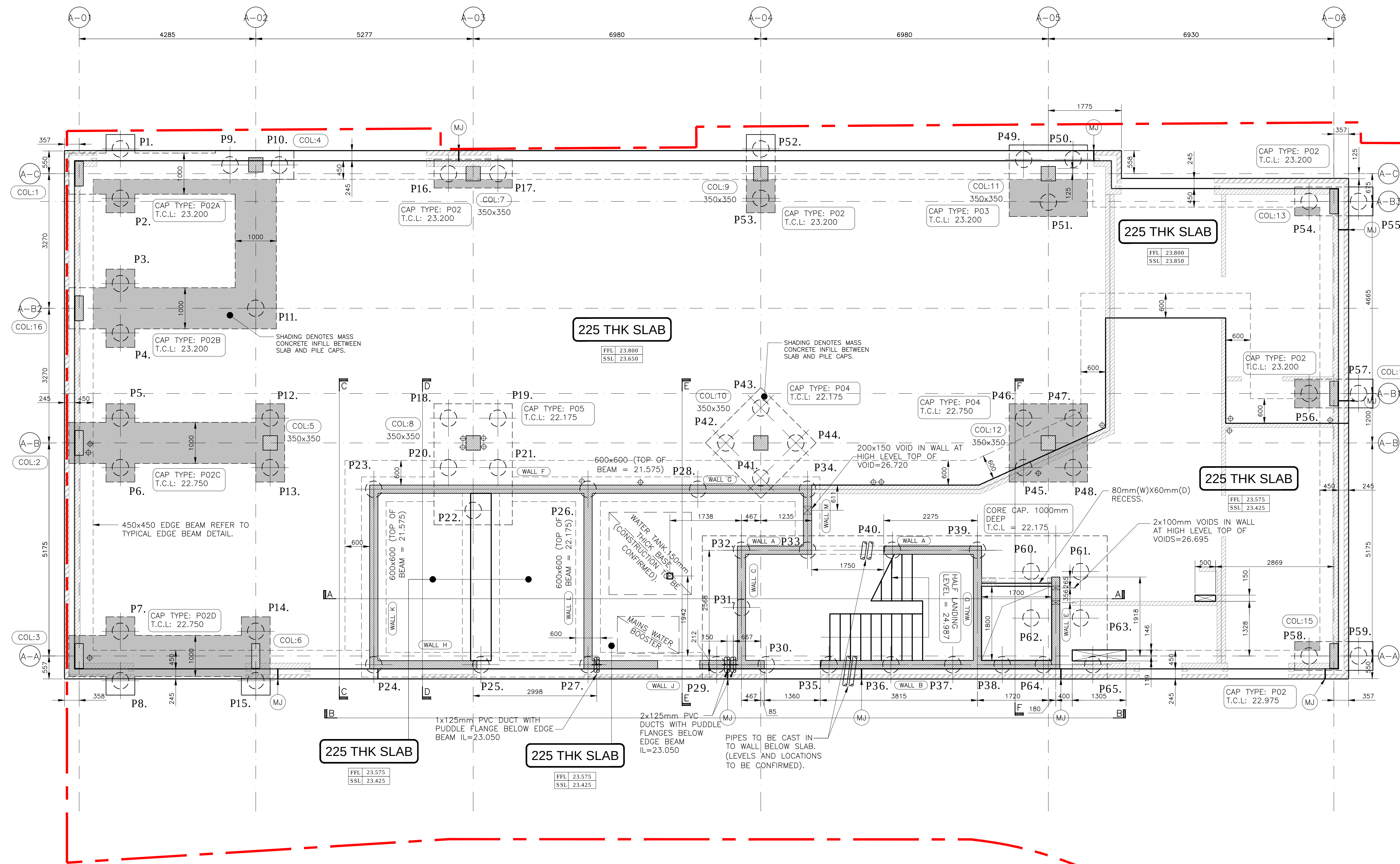
Ground Floor Scale 1:50
