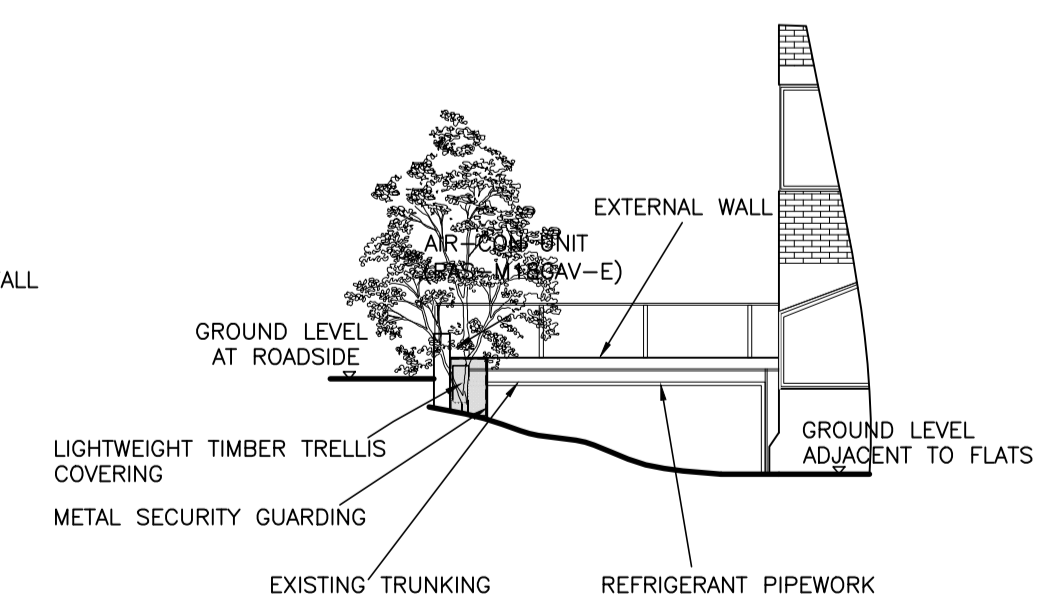
PROPOSED PART FRONT ELEVATION FROM PRINCE ALBERT ROAD 1:100
