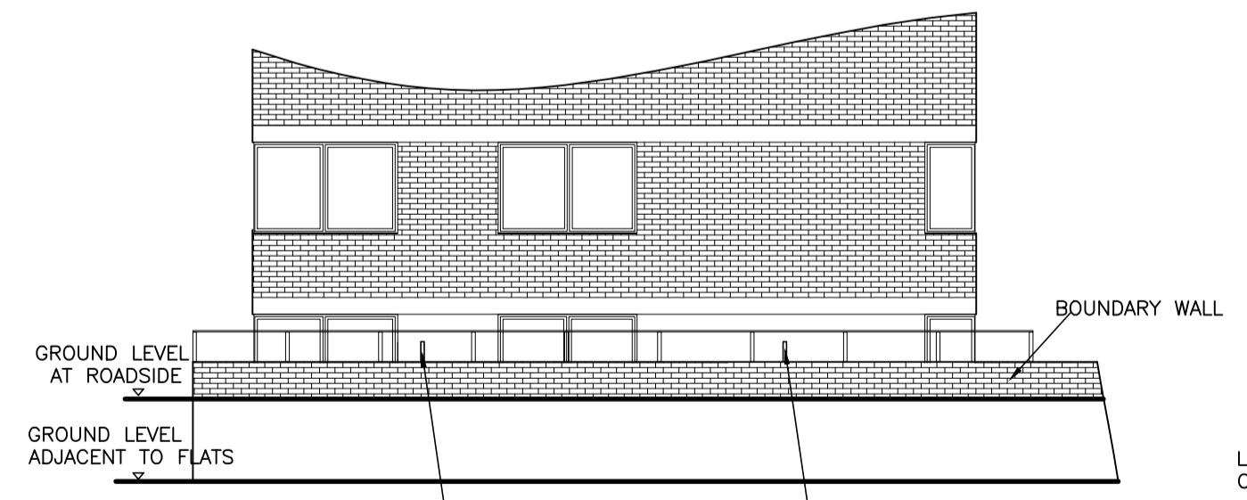
PROPOSED SIDE ELEVATION (FROM ALBERT TERRACE) STREET VIEW 1:100
