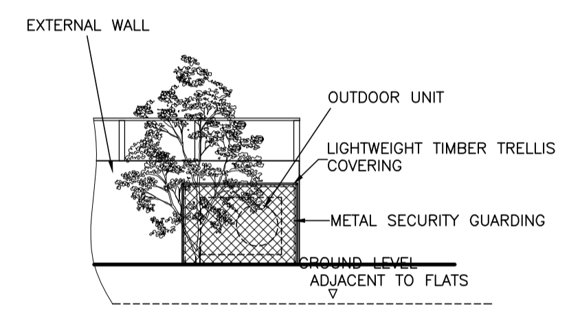
PROPOSED FRONT ELEVATION OF UNIT 1:100
