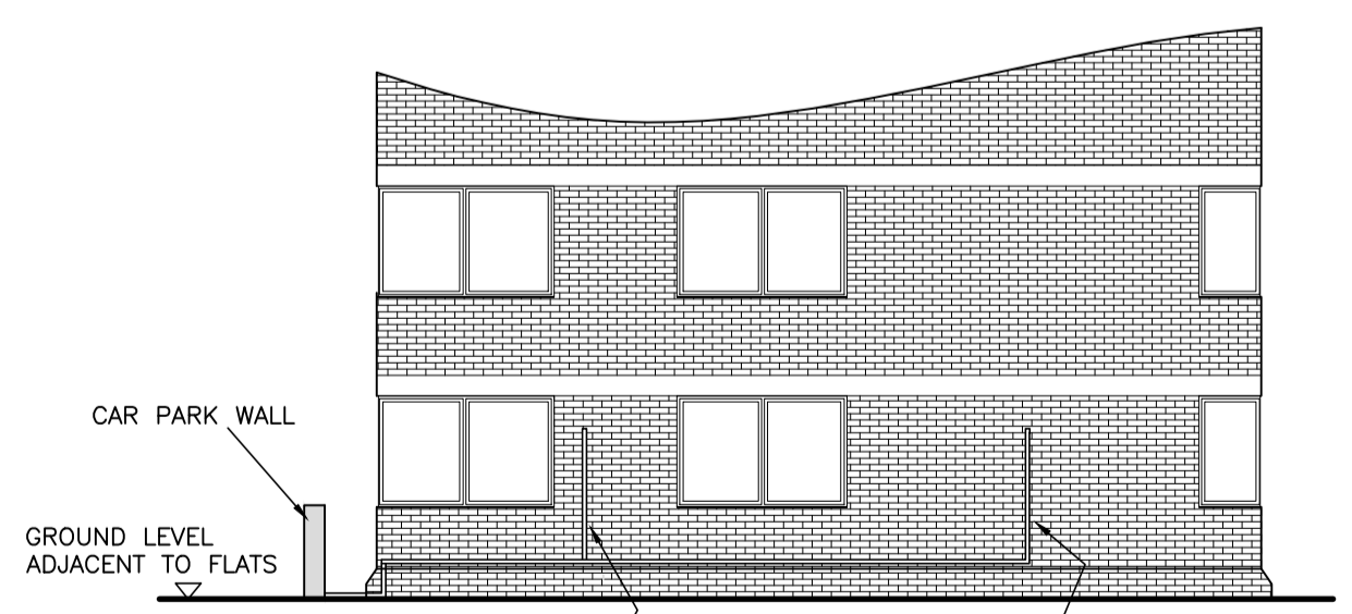
PROPOSED SIDE ELEVATION (FROM WITHIN COMMUNAL GARDEN) 1:100
