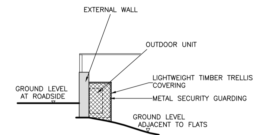
TYPICAL CROSS SECTION 1:50
