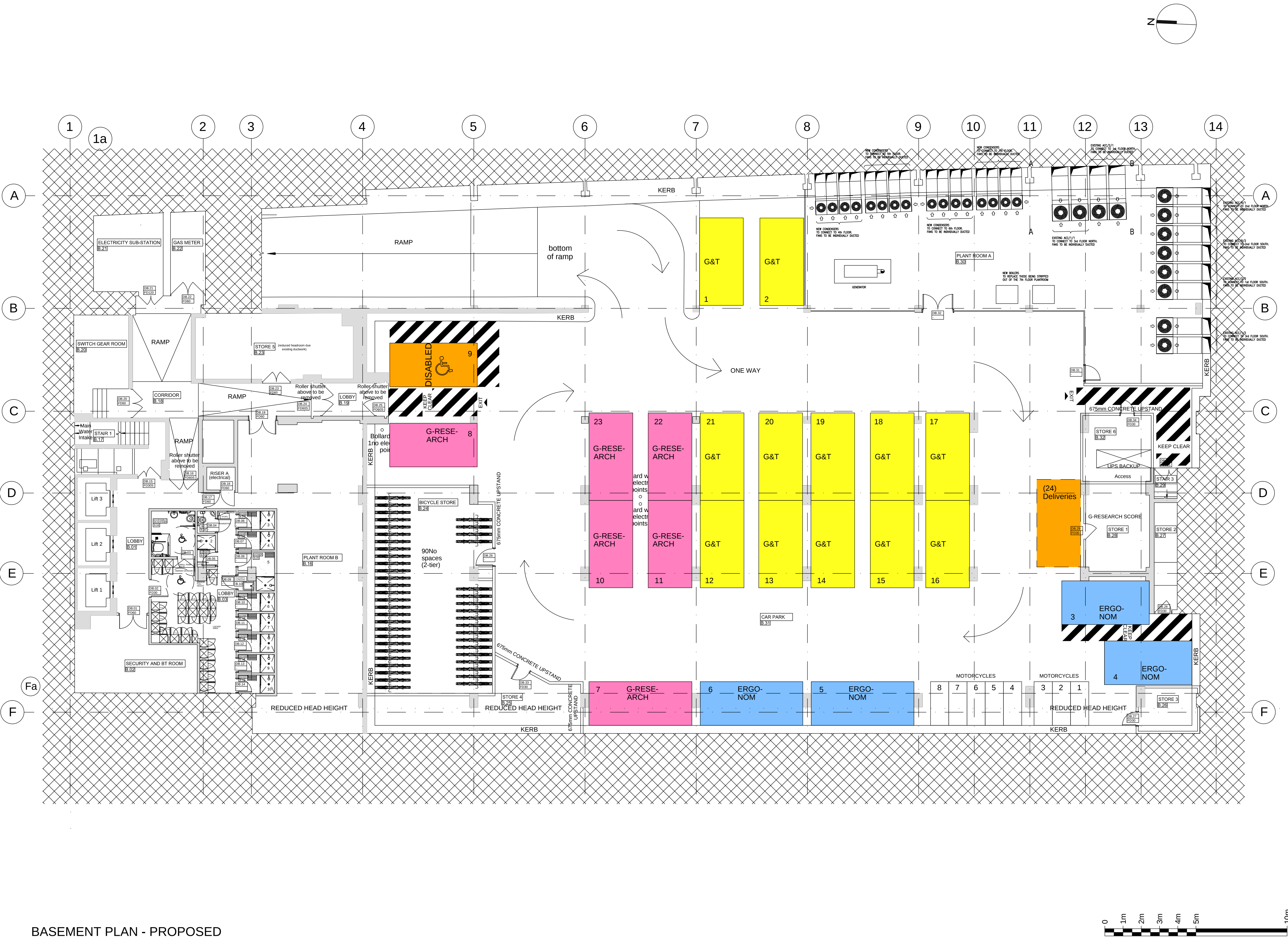
BASEMENT PLAN - PROPOSED
