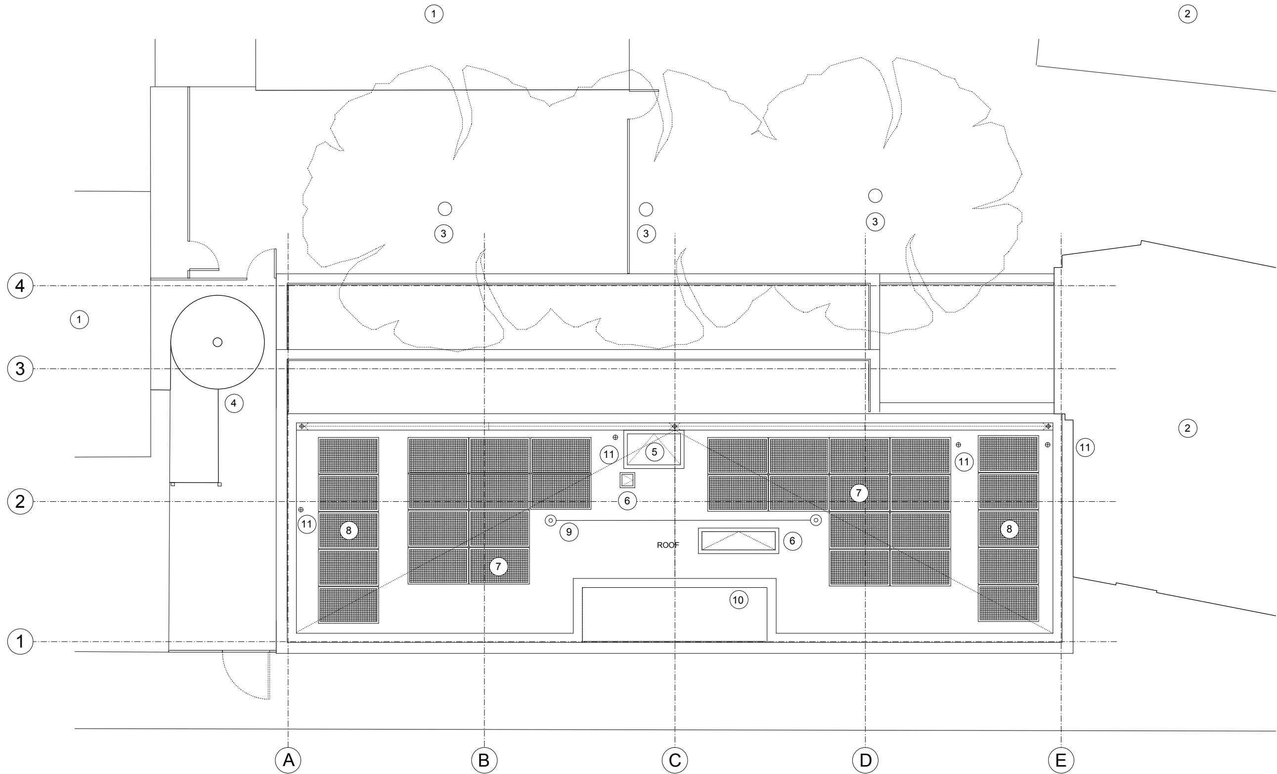
1 PROPOSED FOURTH FLOOR
