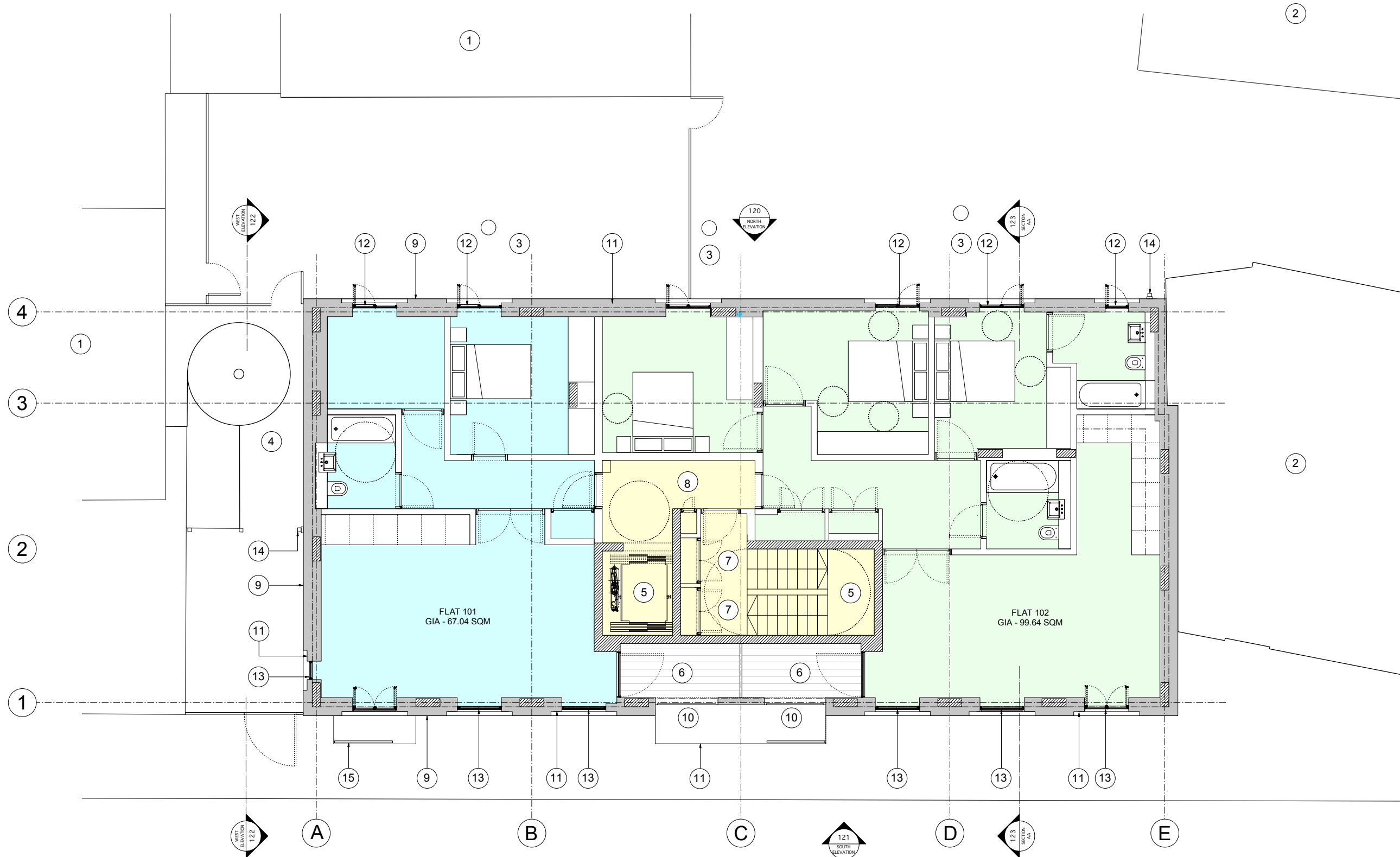
1 PROPOSED FIRST FLOOR
