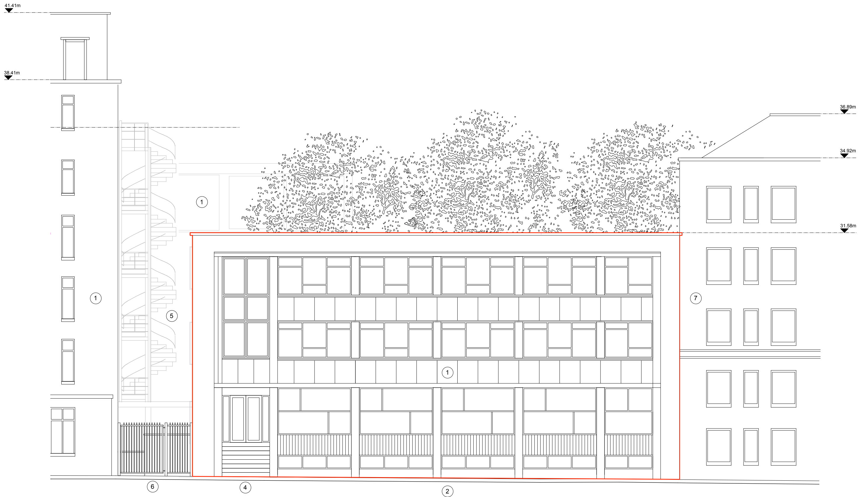
1 EXISTING SOUTH ELEVATION
