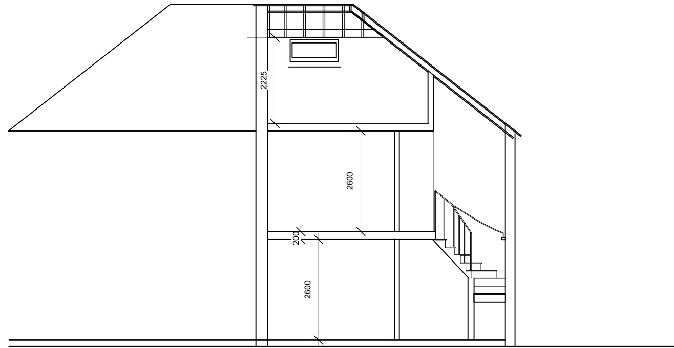
Section AA
