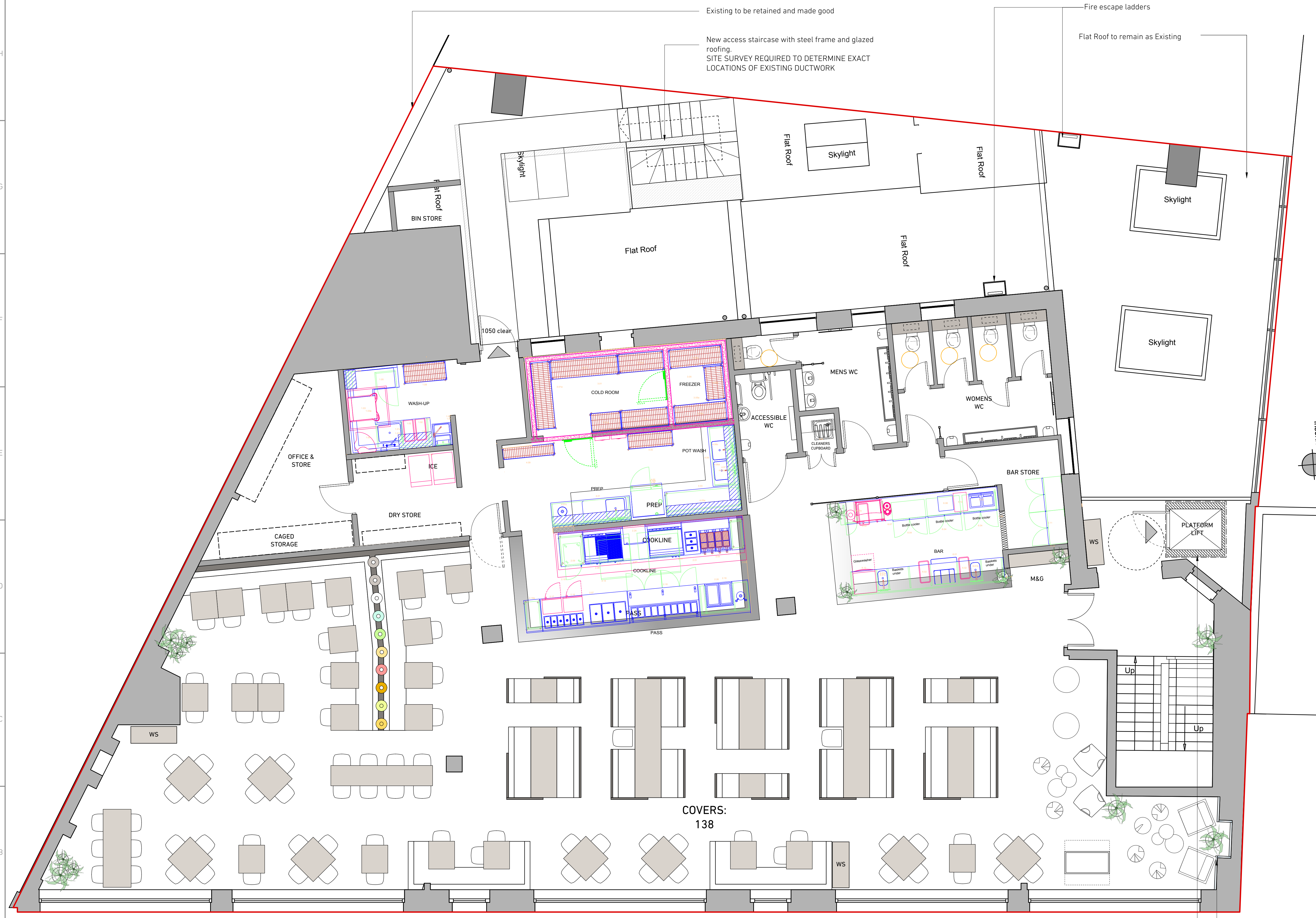
1 PROPOSED FIRST FLOOR GENERAL ARRANGEMENT Scale: 1:50
