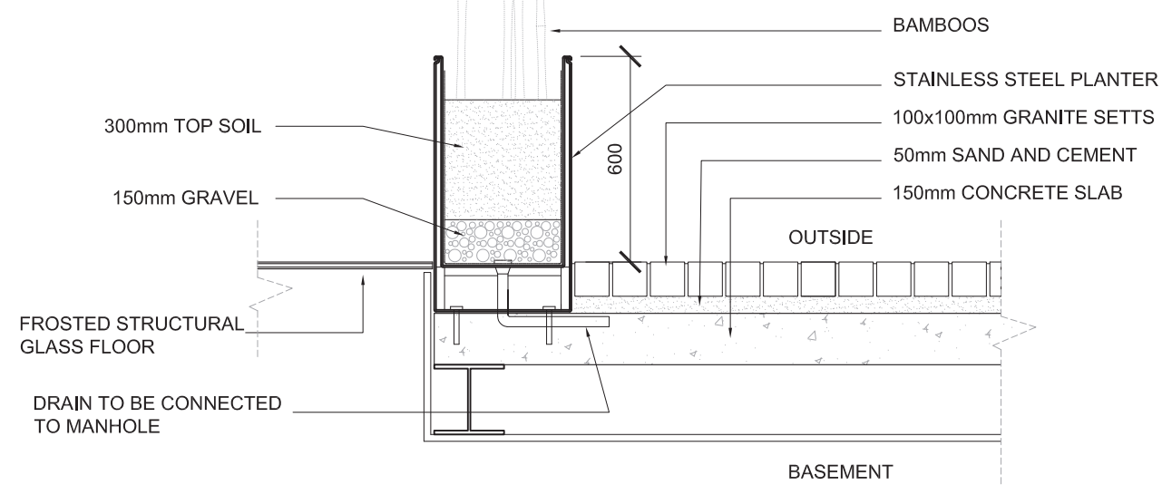
PLANTER DETAIL 02 SCALE 1:20
