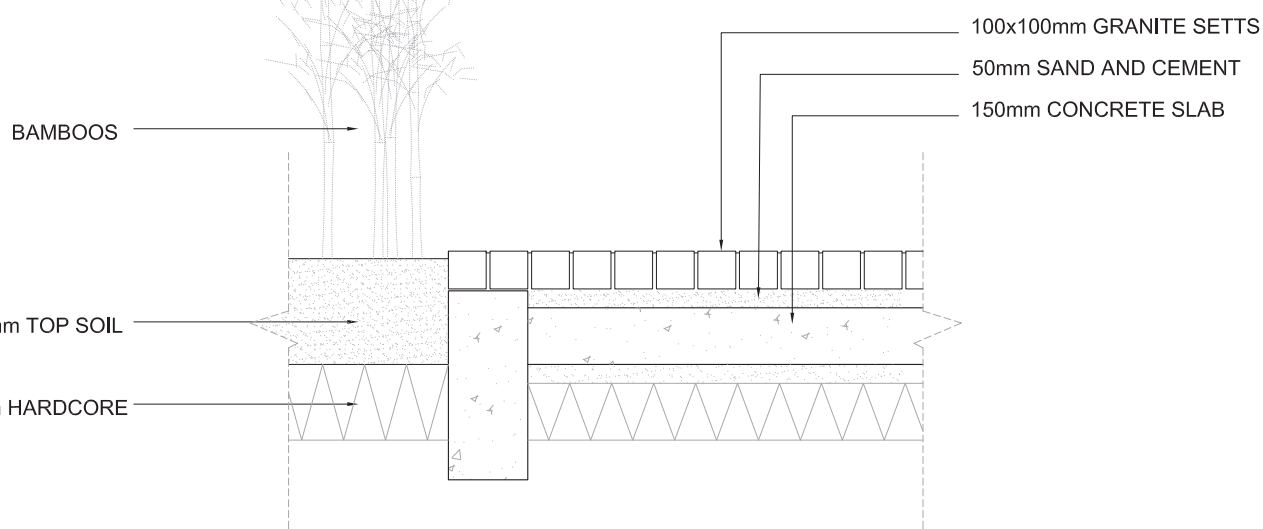
PLANTER DETAIL 01 SCALE 1:20
