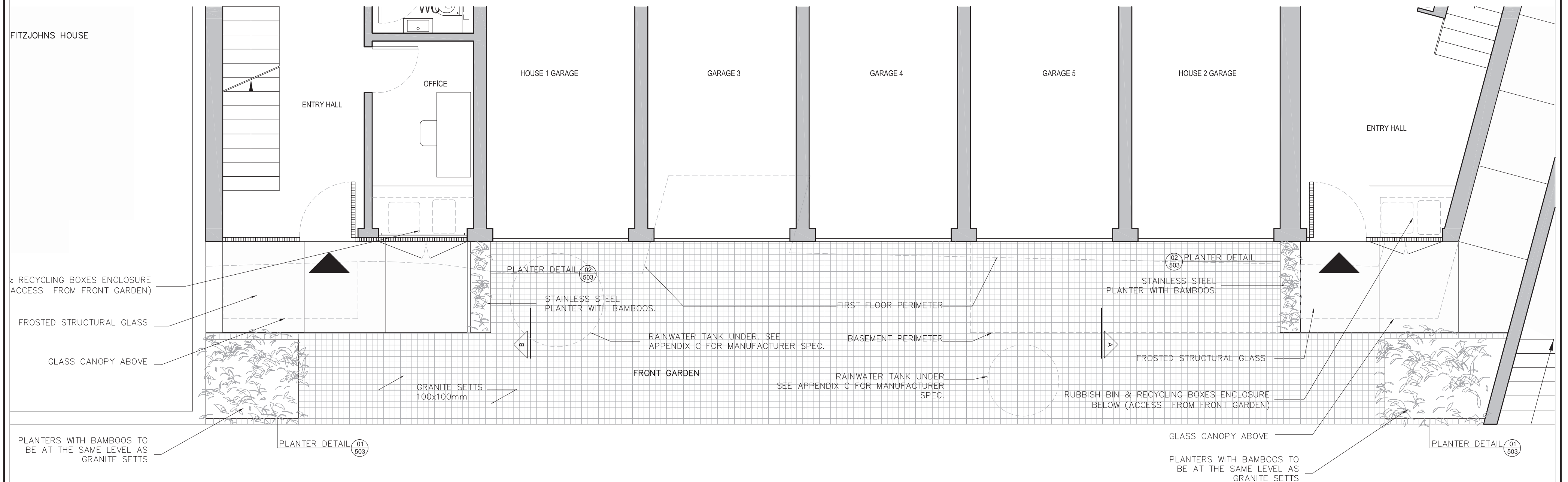
FRONT GARDEN PLAN SCALE 1:50
