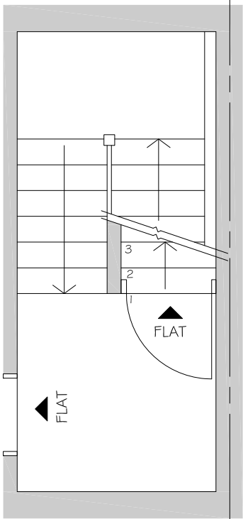
Existing Lower Level Landing Arrangement
