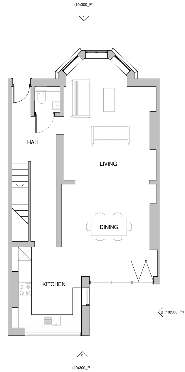
Lower Ground Floor 1 : 50
