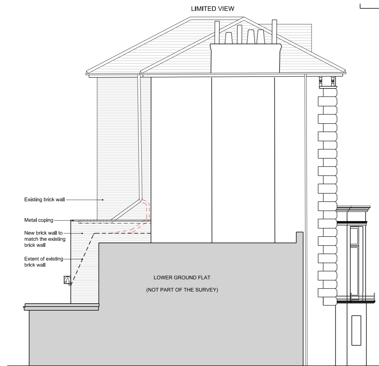
SIDE ELEVATION
