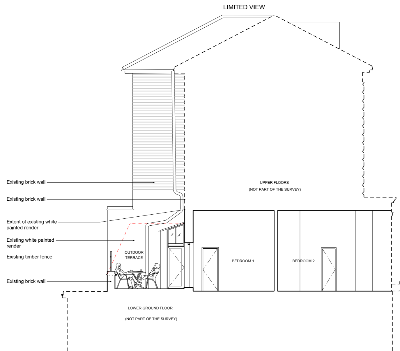
EXISTING REAR SECTION C
