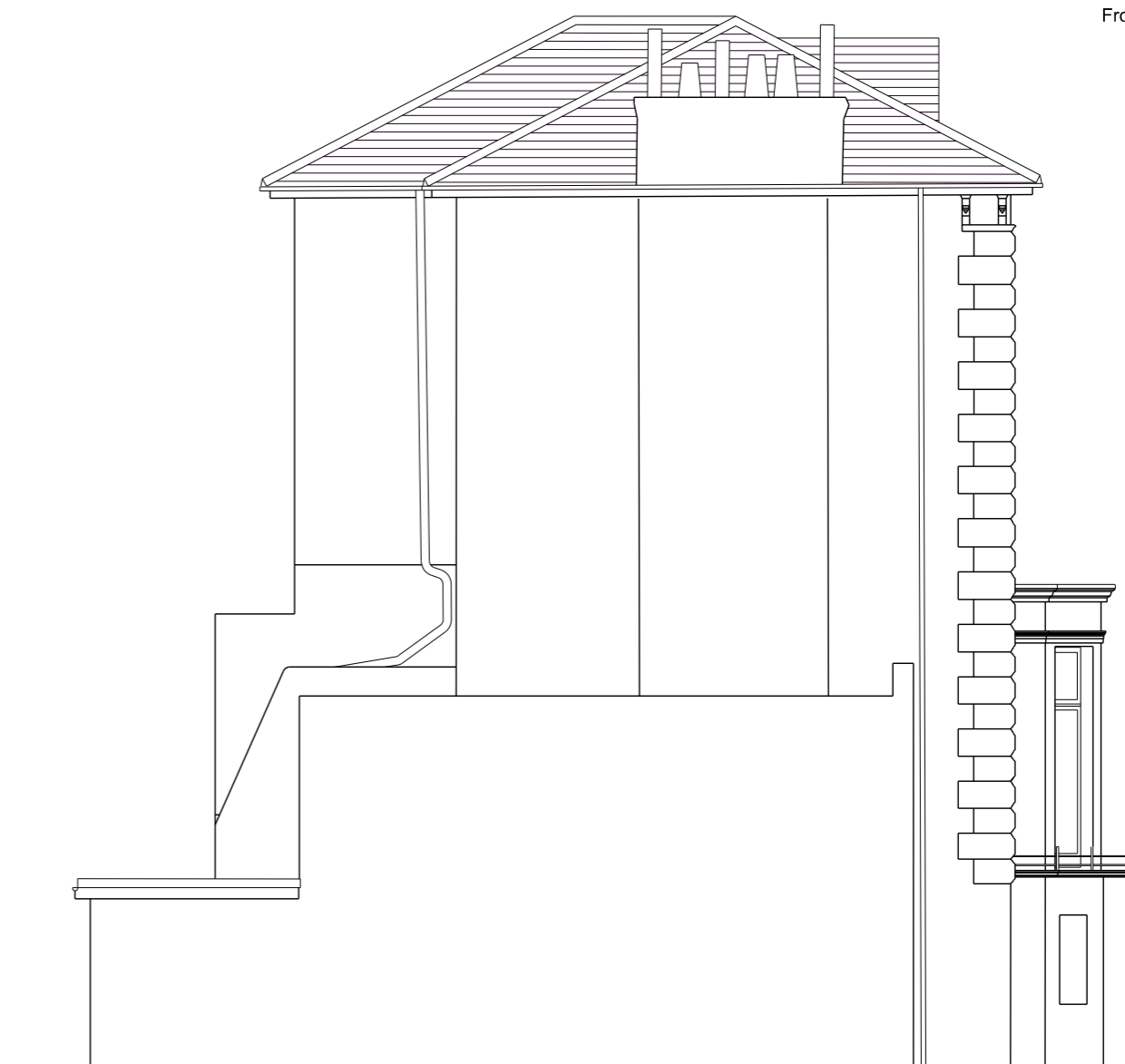
SIDE ELEVATION
