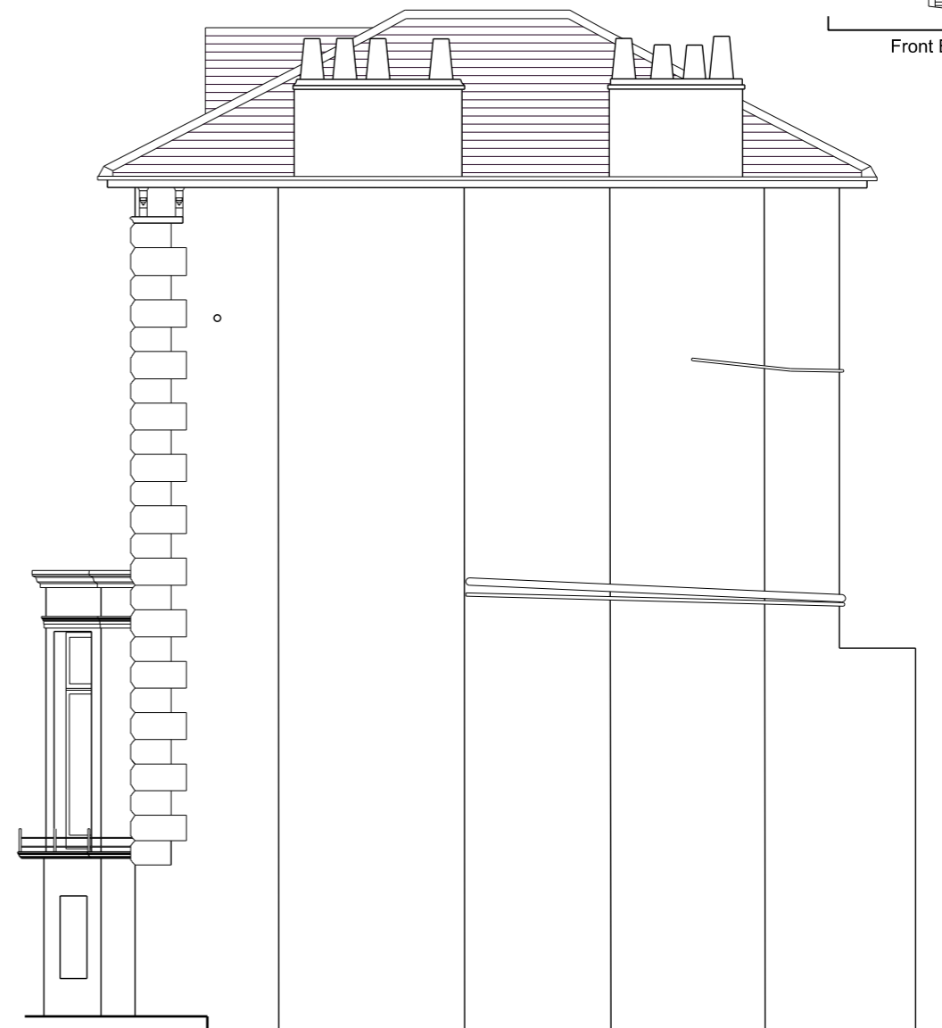
SIDE ELEVATION
