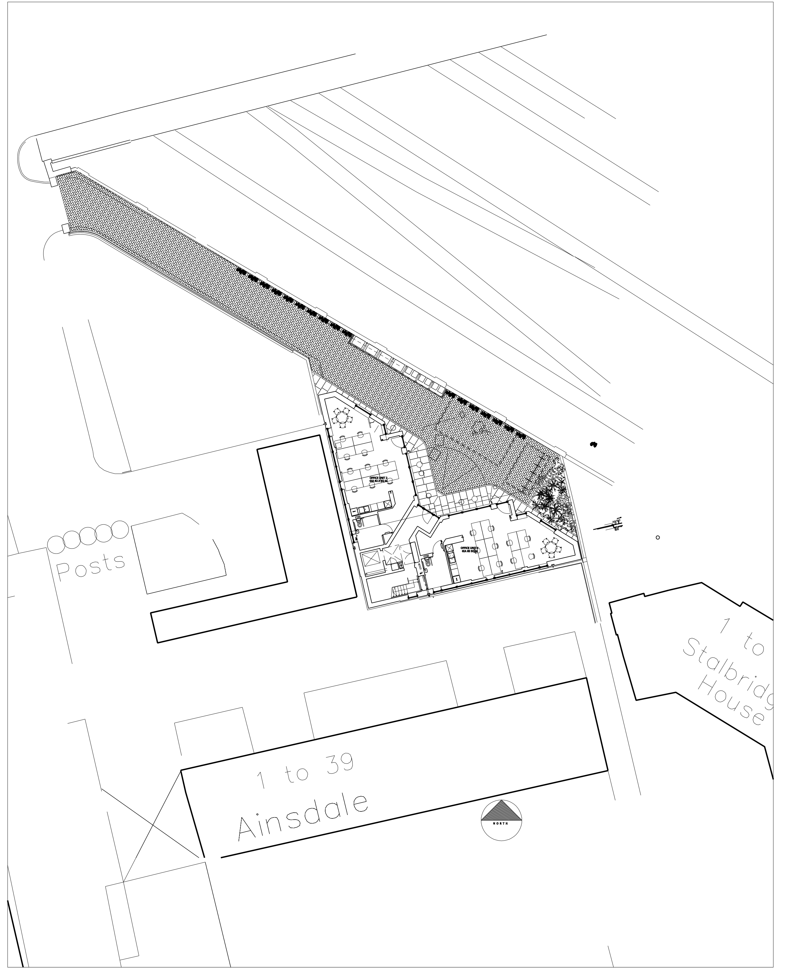
SITE PLAN AT GROUND FLOOR LEVEL
