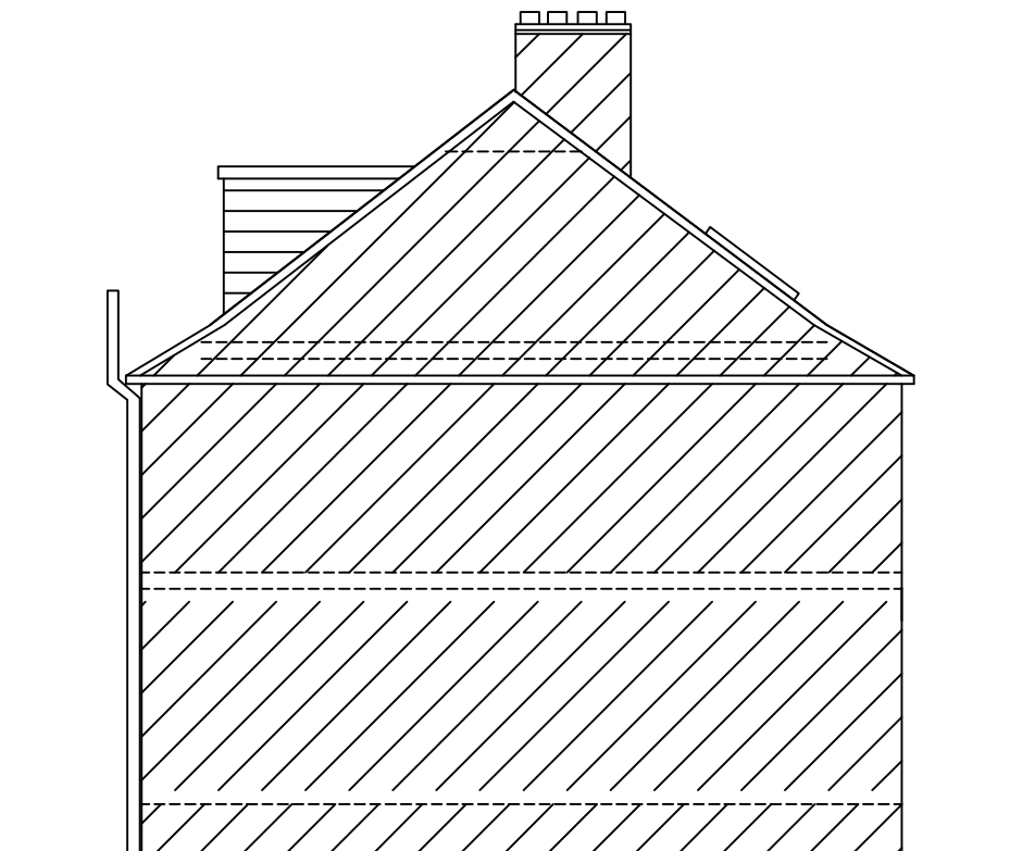
Proposed Attached Elevation
