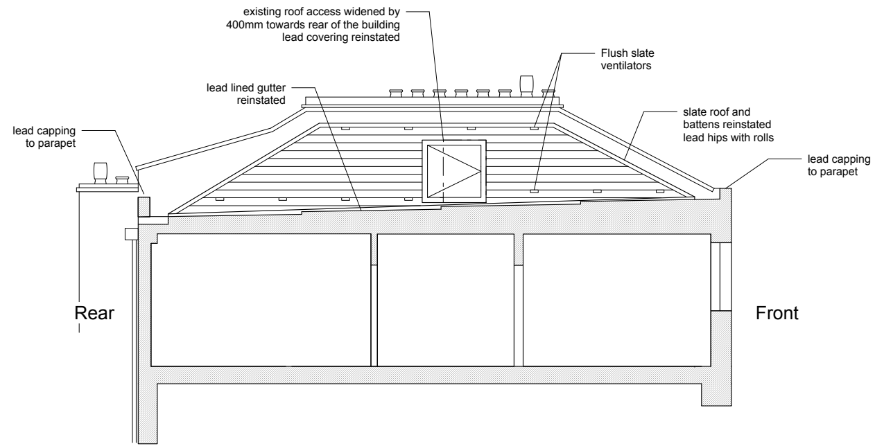
B Proposed Section B 12 1:50@A1, 1:100@A3
