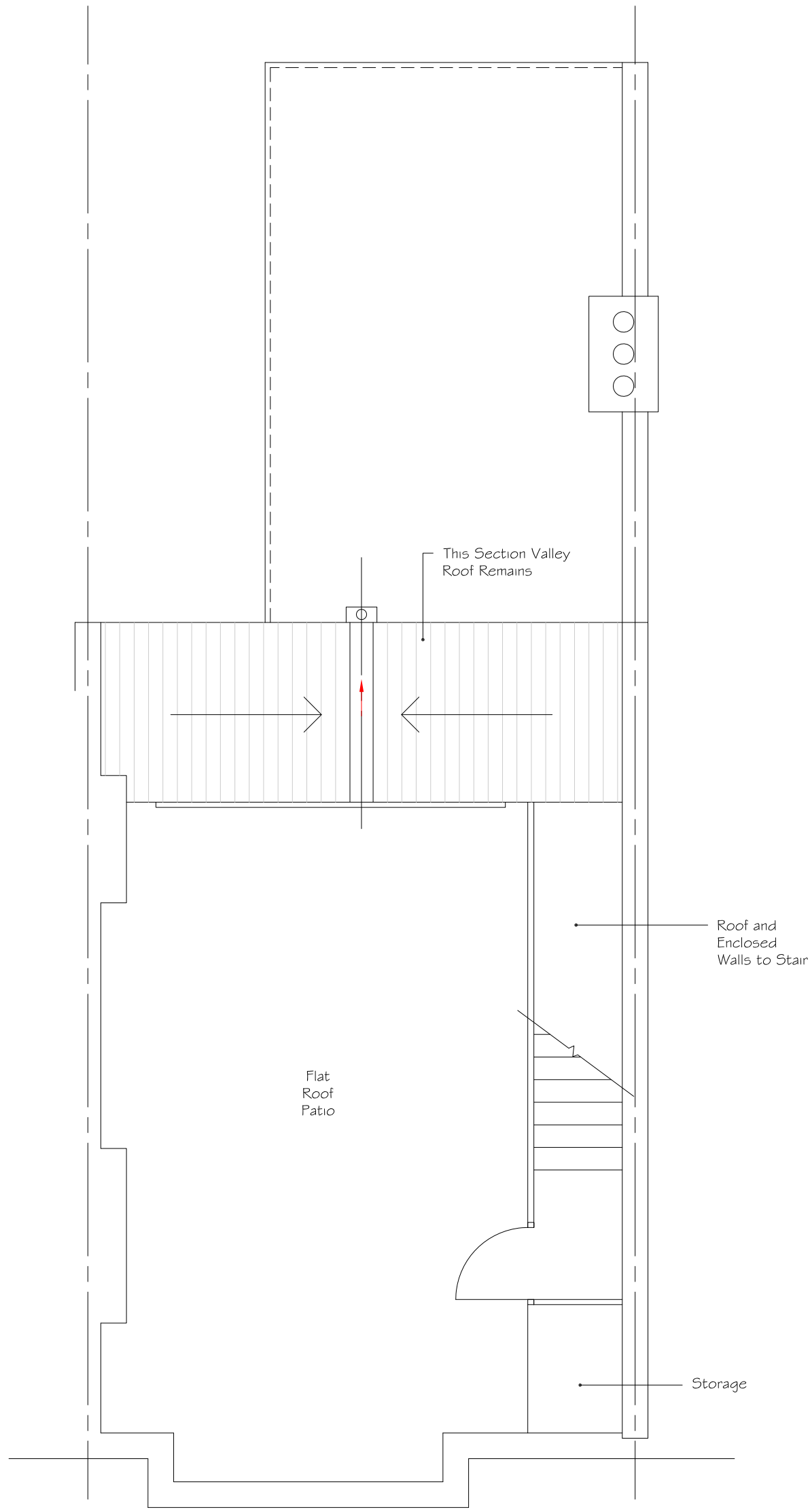
PROPOSED ROOF GARDEN Scale 1:50
