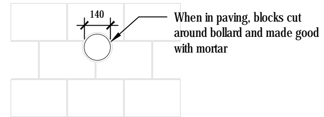
2 Bollard plans
