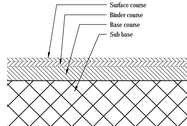
5 Section - Black tarmac Q22:145
