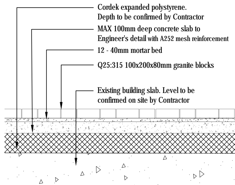
3 Section - Granite Blocks
