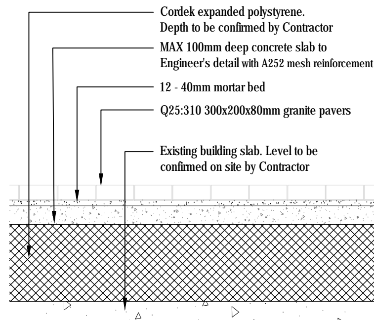
4 Section - Granite pavers
