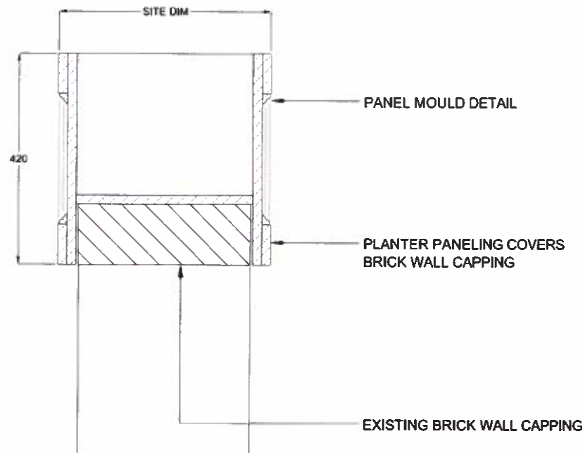
D1 PROPOSED PLANTER BOX SCALE 1:10
