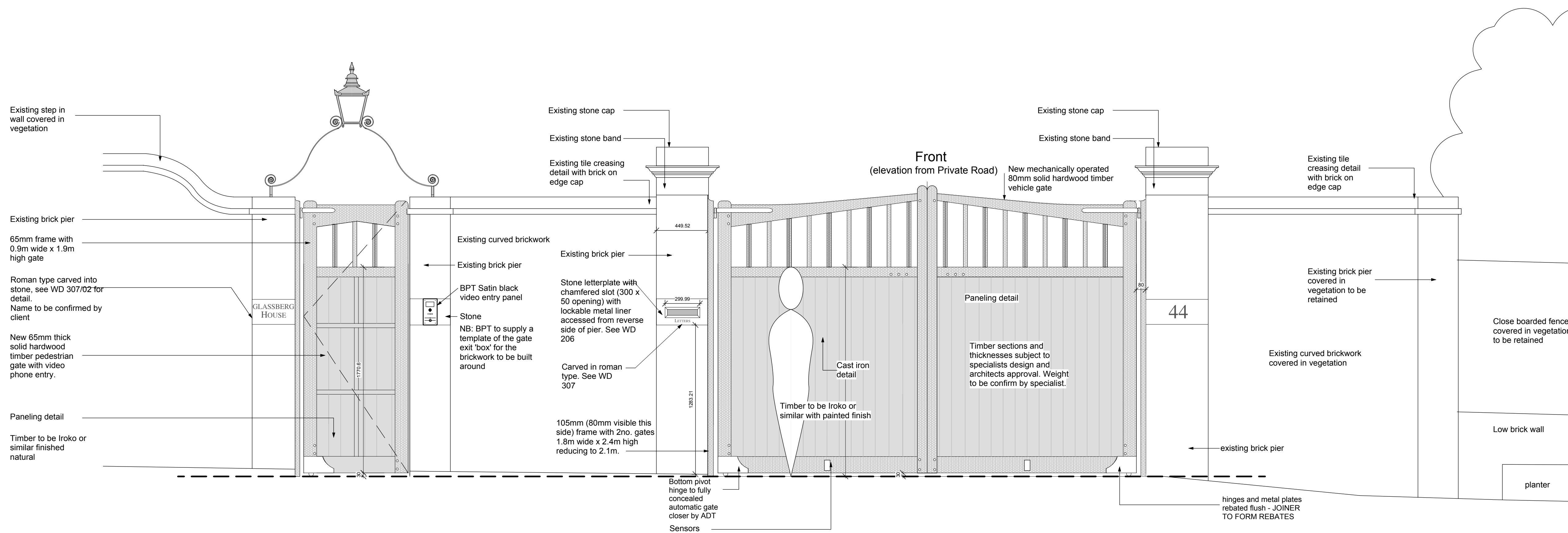
Elevation From Private Road 1:20 Scale @A1
