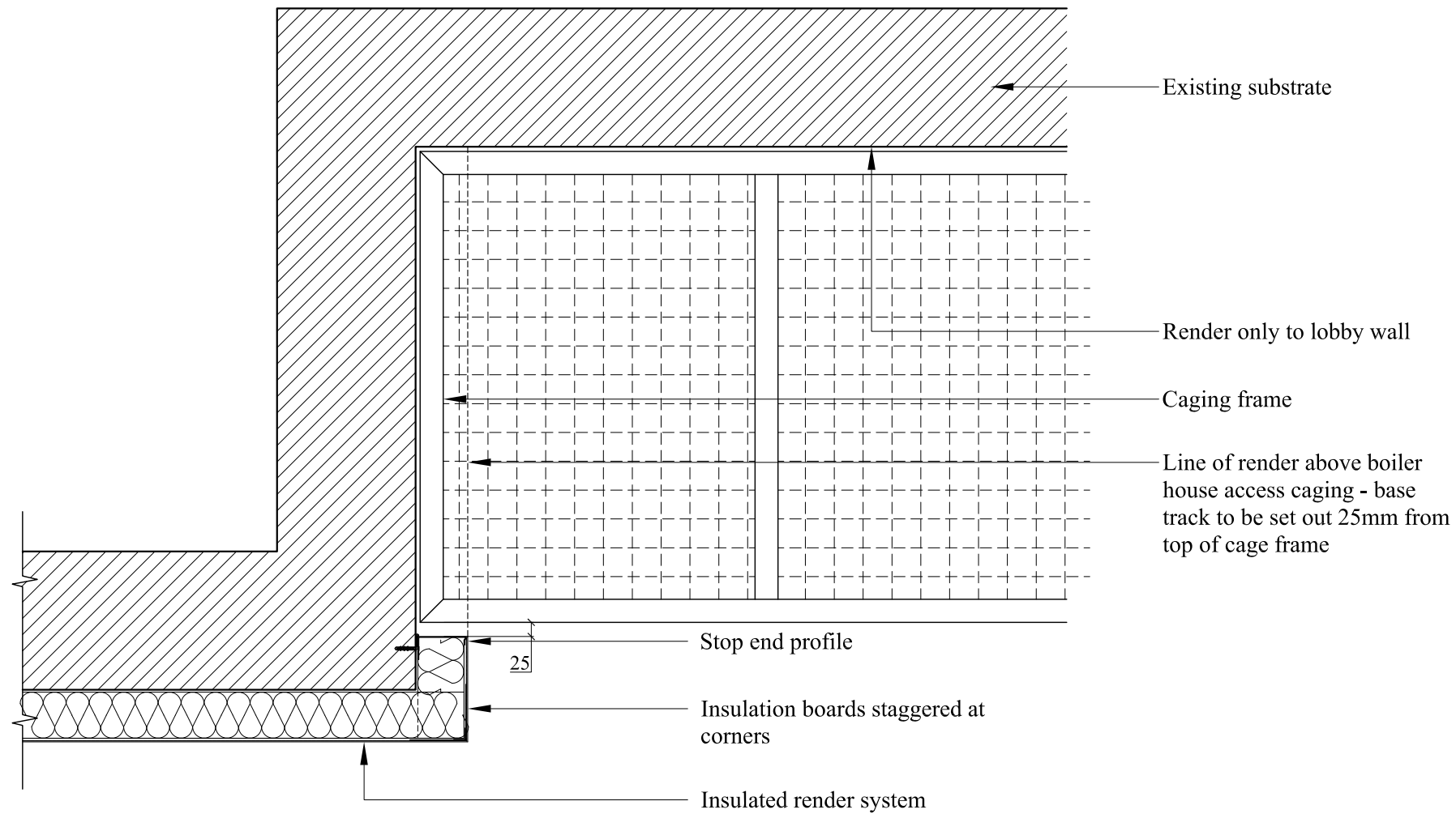
SECTION THROUGH PROTECTIVE CAGING TO BOILER ACCESS STAIR
