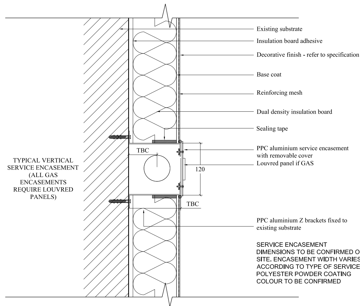
VERTICAL SERVICE ENCASEMENT DETAIL
