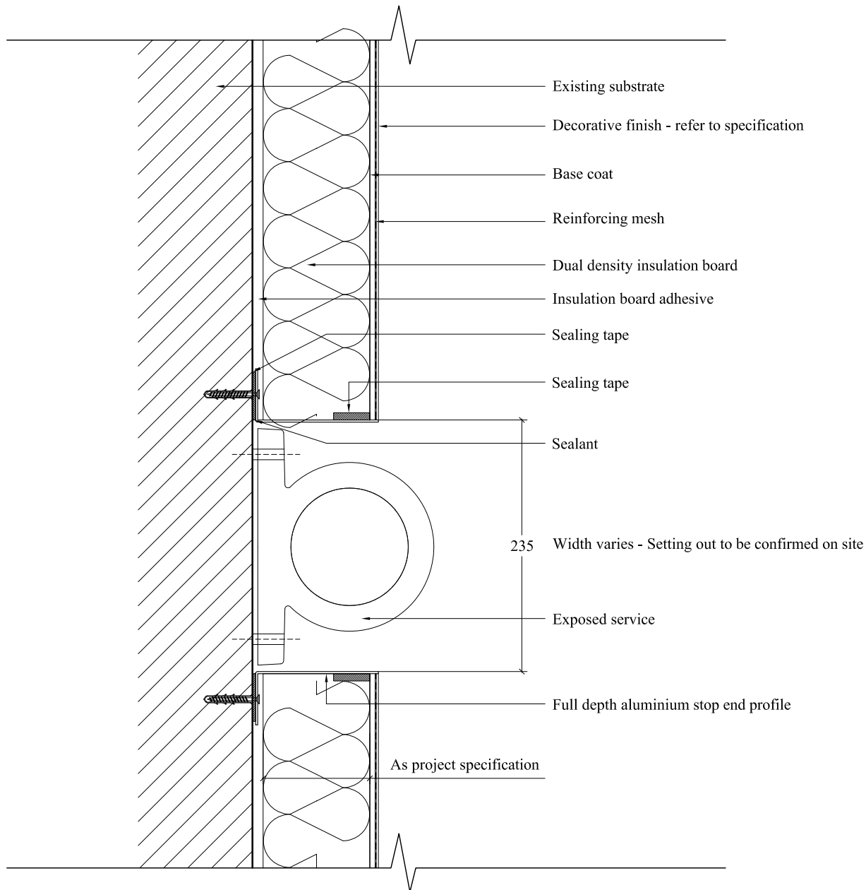
SECTION THROUGH EXPOSED SERVICE PIPE
