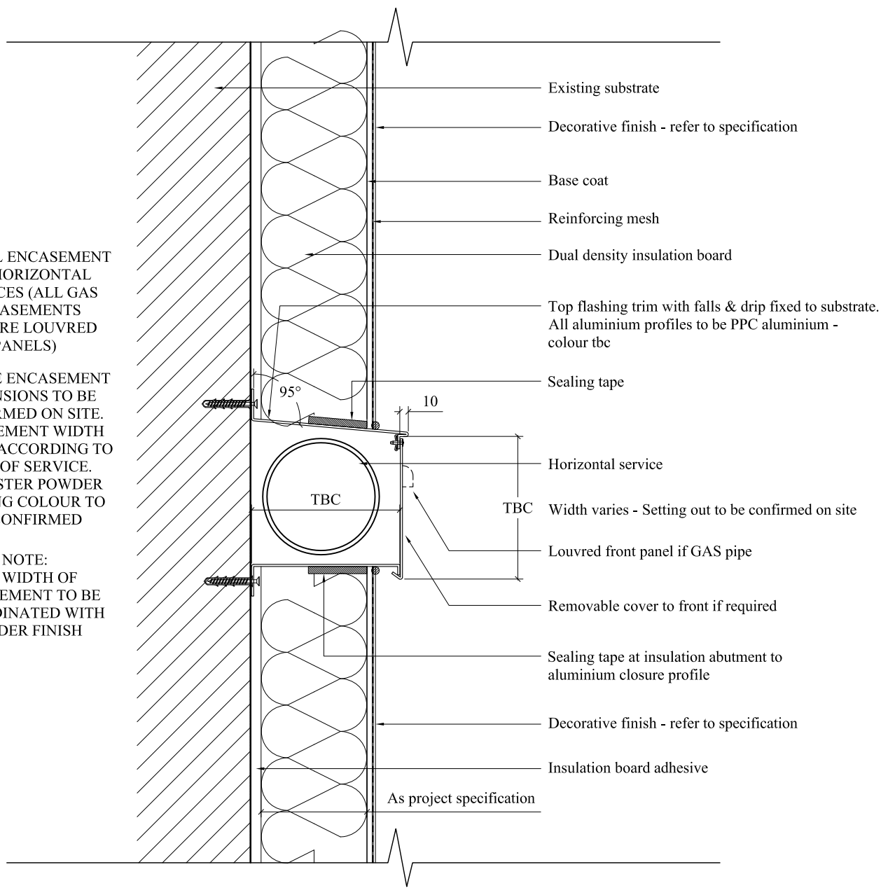
SECTION THROUGH HORIZONTAL SERVICE ENCASMENT
