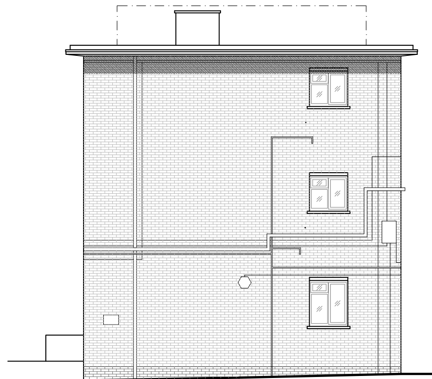
ELEVATION M
