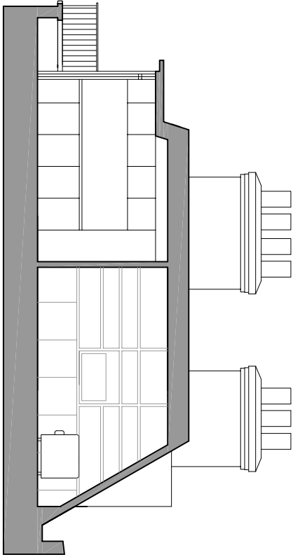
PROPOSED SECTION: BB
