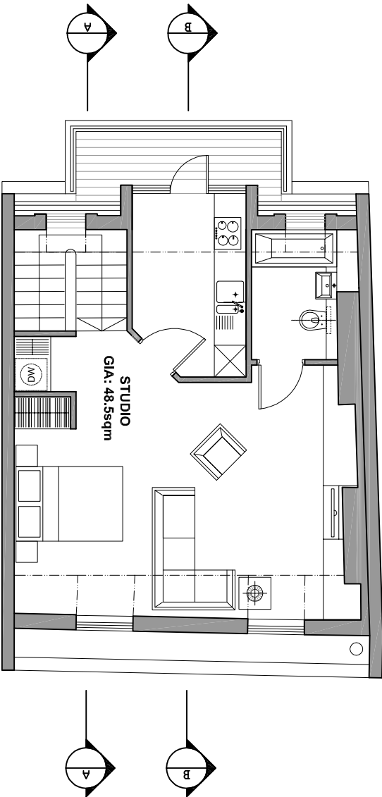
FOURTH FLOOR
