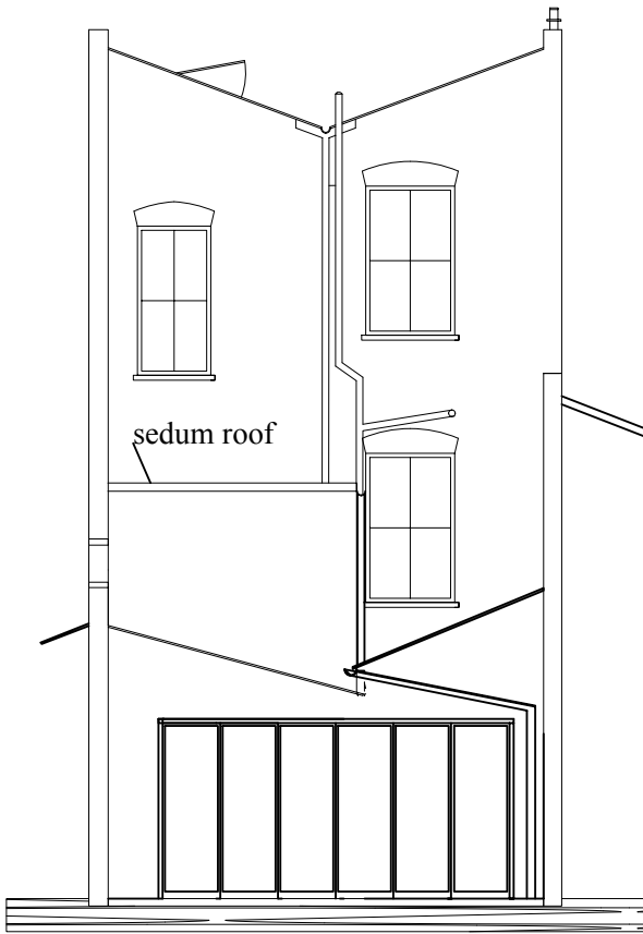
REAR ELEVATION
