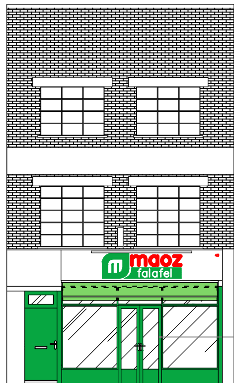
FRONT ELEVATION (as existing)
