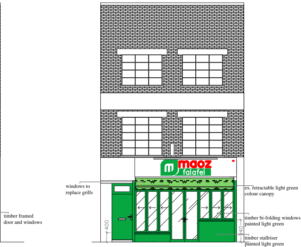
FRONT ELEVATION (as proposed)
