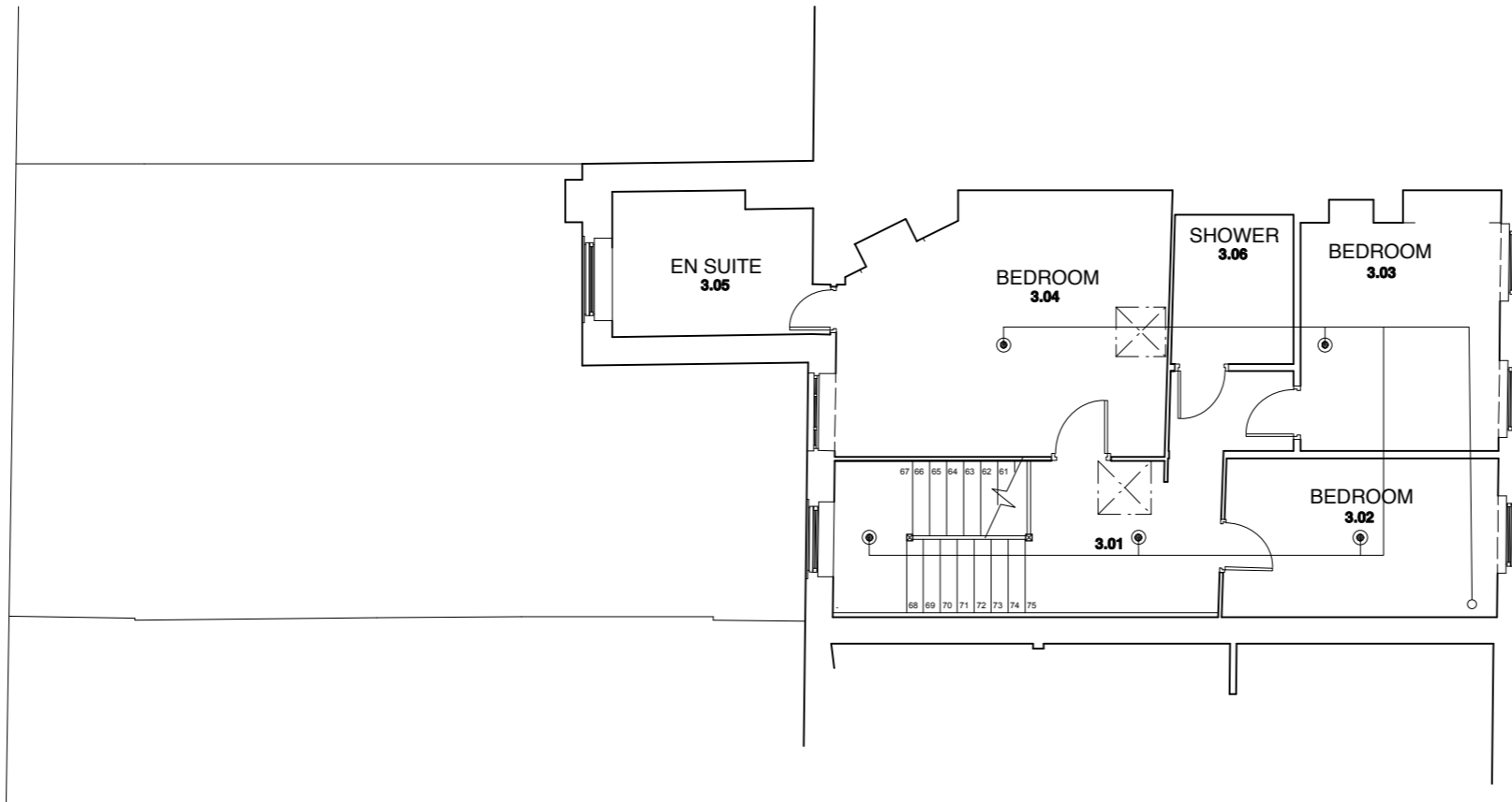
PROPOSED THIRD FLOOR PLAN SHOWING SPRINKLER LAYOUT. LAYOUT TO BE COORDINATED WITH ROOF JOIST LAYOUT
