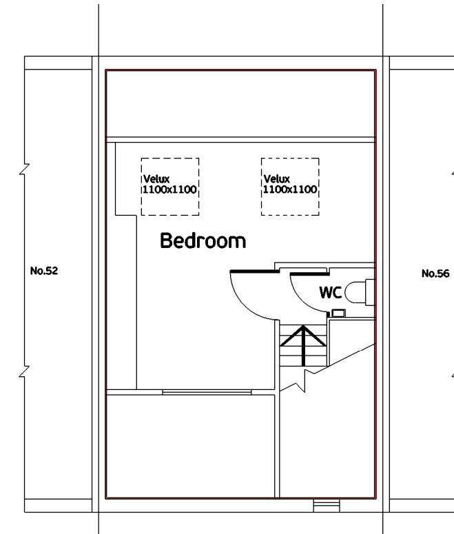
Third floor
