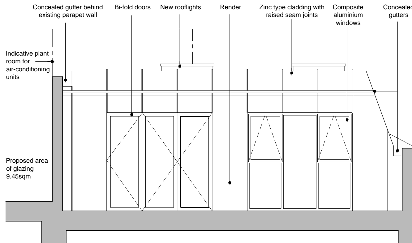
GRAFTON WAY SECTIONAL ELEVATION
