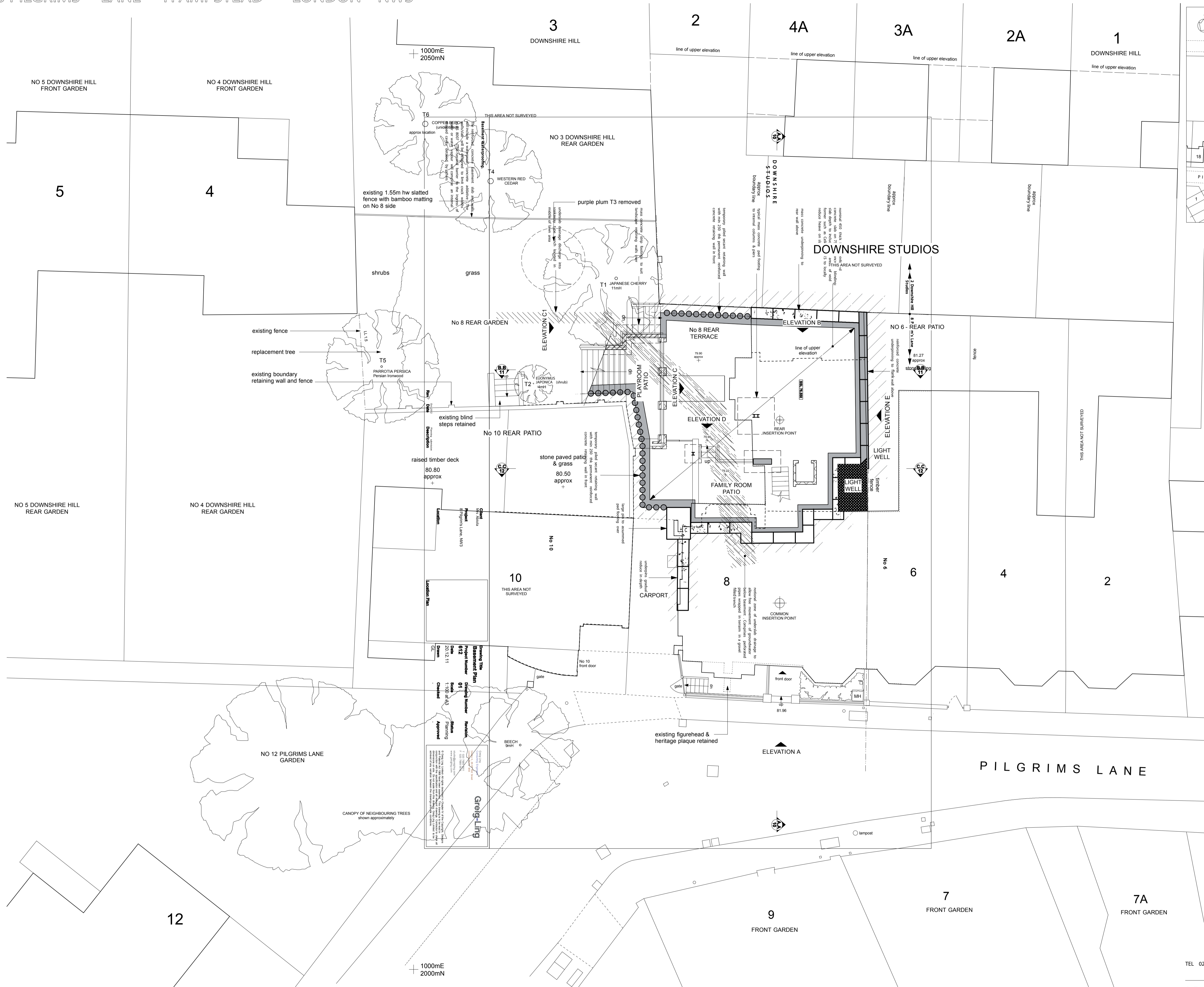
SITE PLAN - PROPOSED - 1:100
