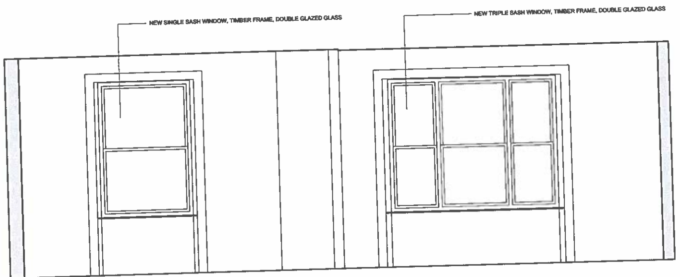
2 PROPOSED ELEVATION BB SCALE 1:50 @ A4
