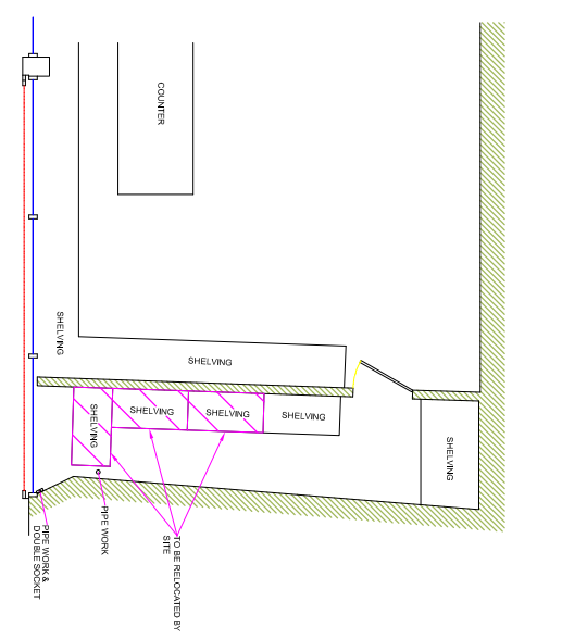
EXISTING (PART) PLAN
