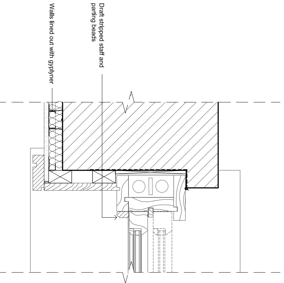
04 - New window - Jamb detail As Proposed
