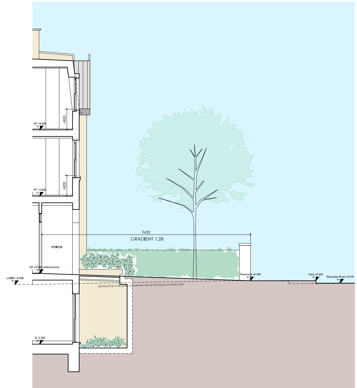
SECTION THROUGH ENTRANCES TO 18-20 ELSWORTHY RD - AS PROPOSED
