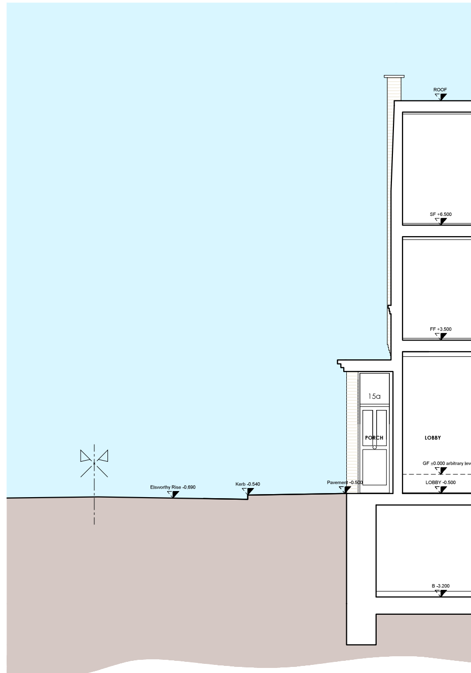
SECTION THROUGH ENTRANCES TO 15A ELSWORTHY RISE - AS PROPOSED
