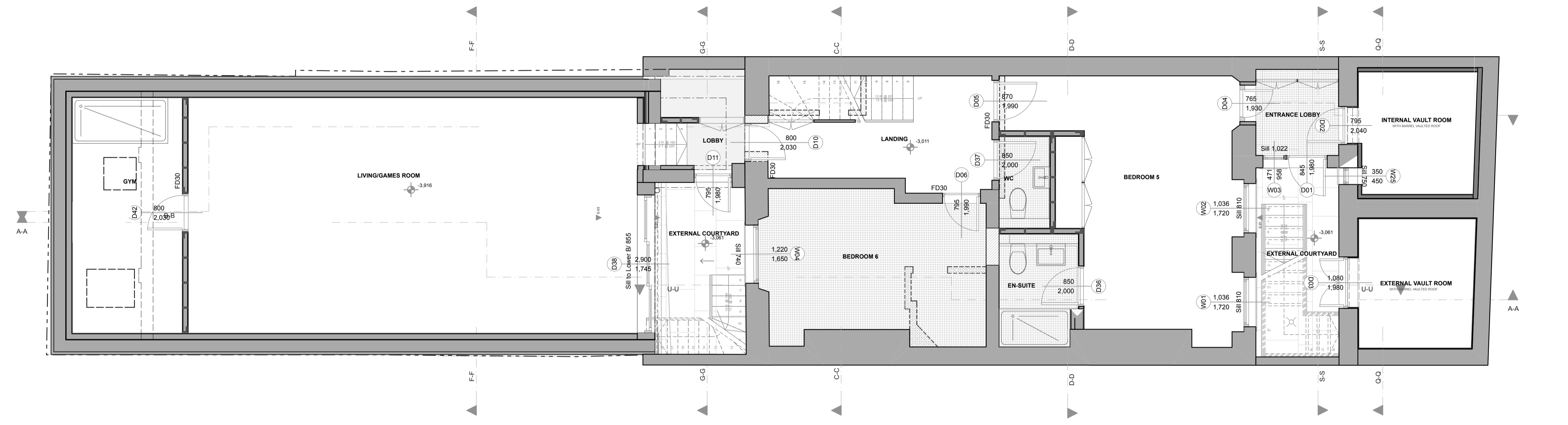
Basement Layout 1:50
