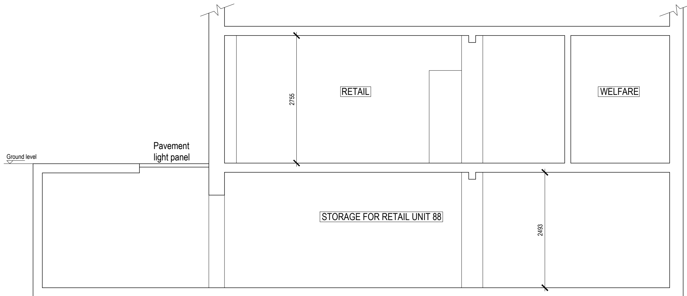
Proposed Section B-B
