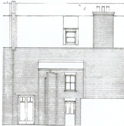
Rear Elevation existing
