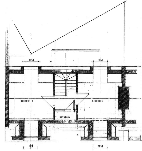
Second Floor proposed
