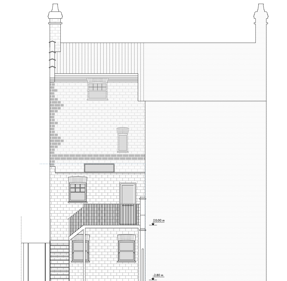
Existing Rear Elevation 1:100 @A3
