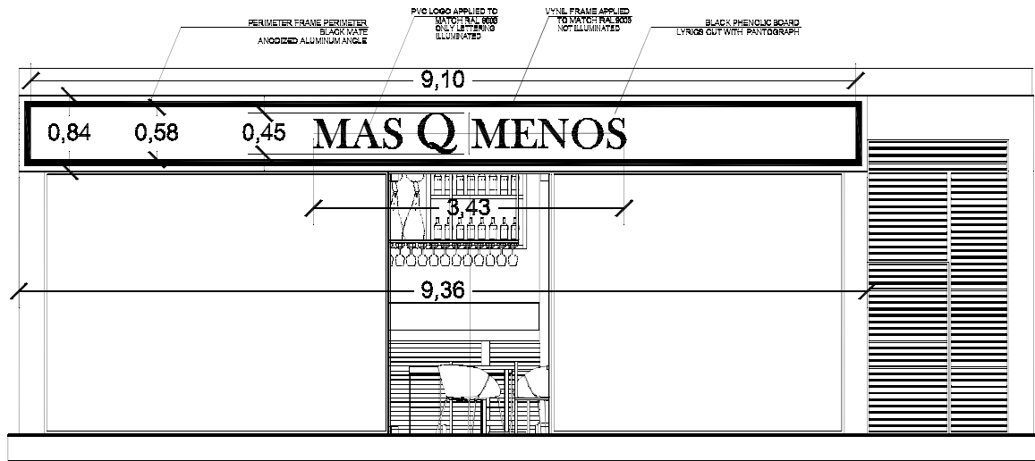
Main Facade
