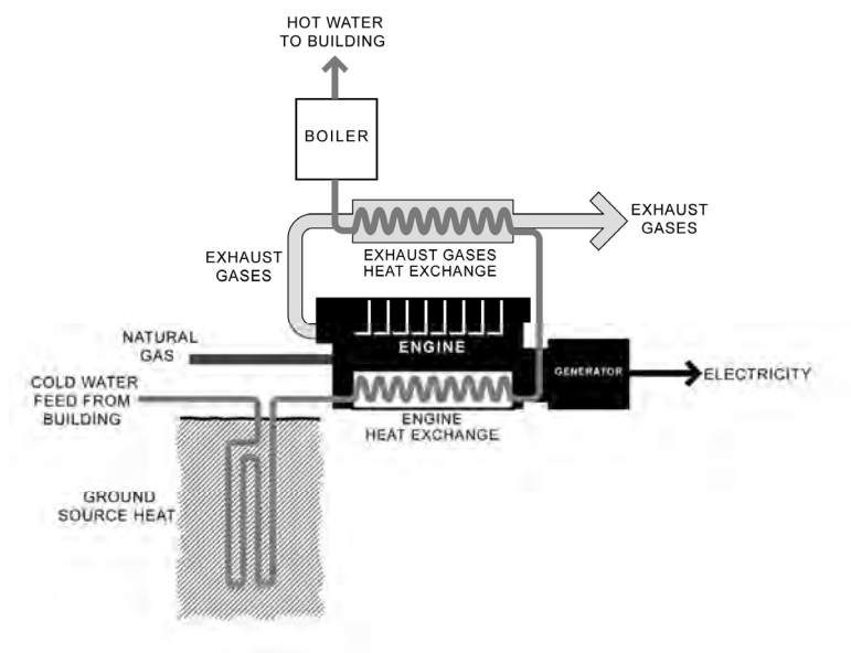
Figure 2. Combined Heat and Power Schematic
