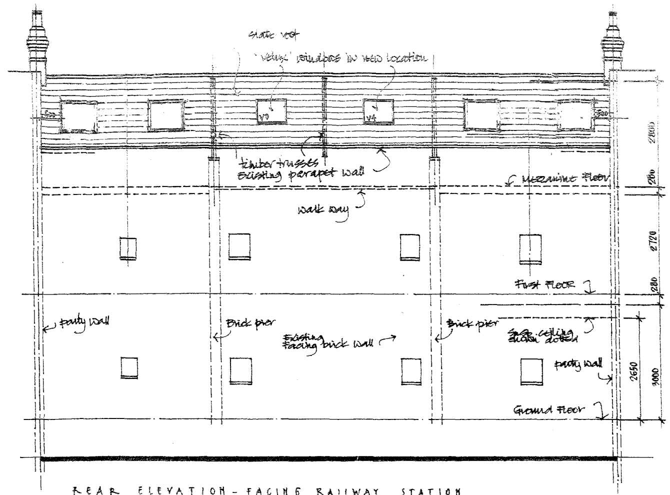
REAR ELEVATION - FACING RAILWAY STATION
