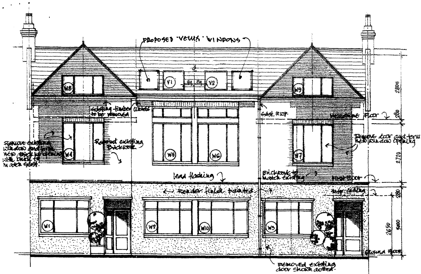
FRONT ELEVATION
