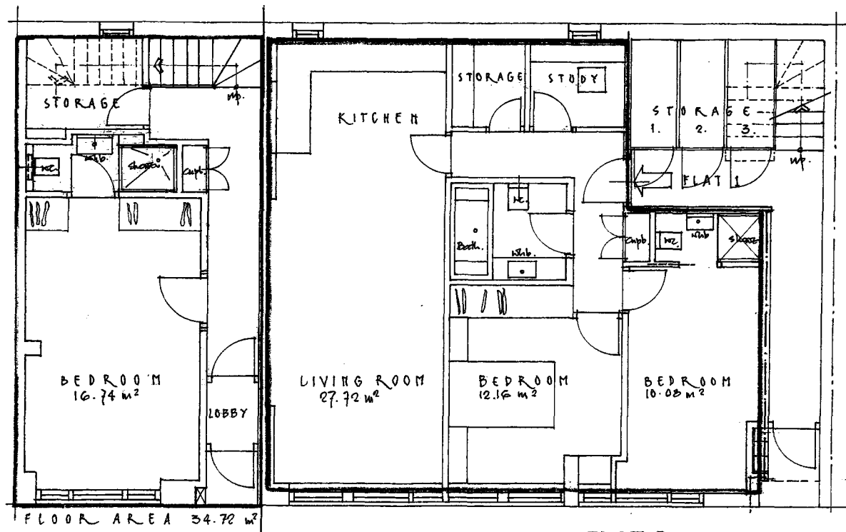
GROUND FLOOR FLAT 1
