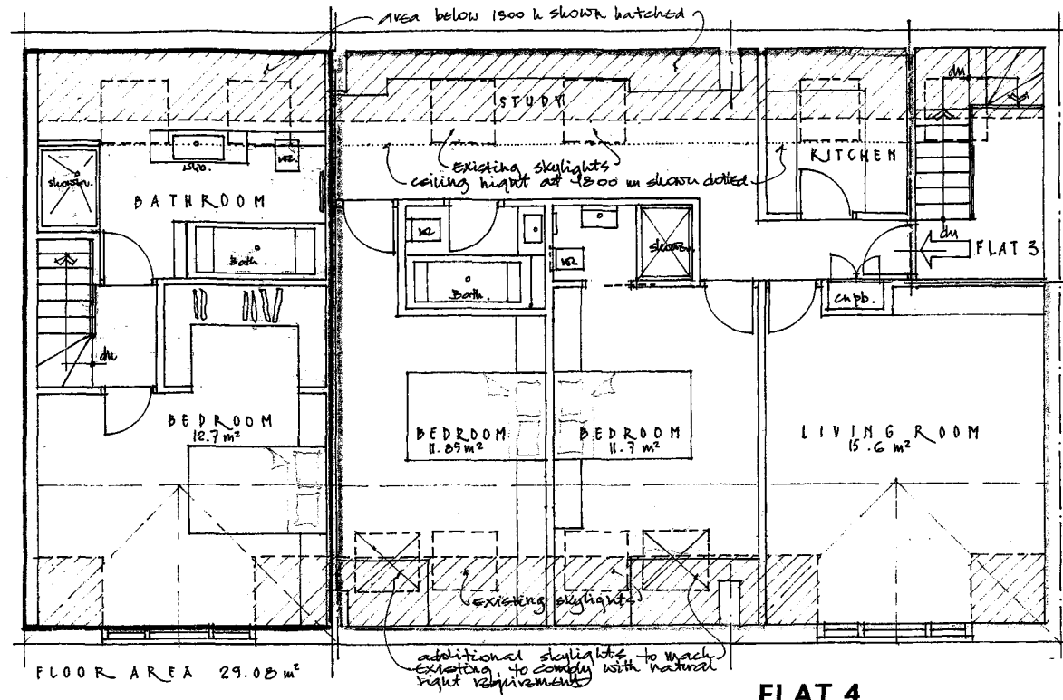
SECOND FLOOR FLAT 4
