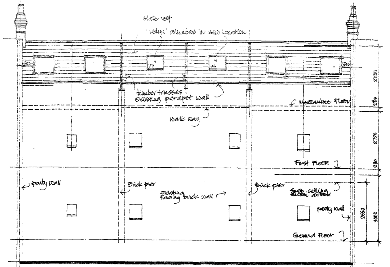
REAR ELEVATION - FACING RAILWAY STATION
